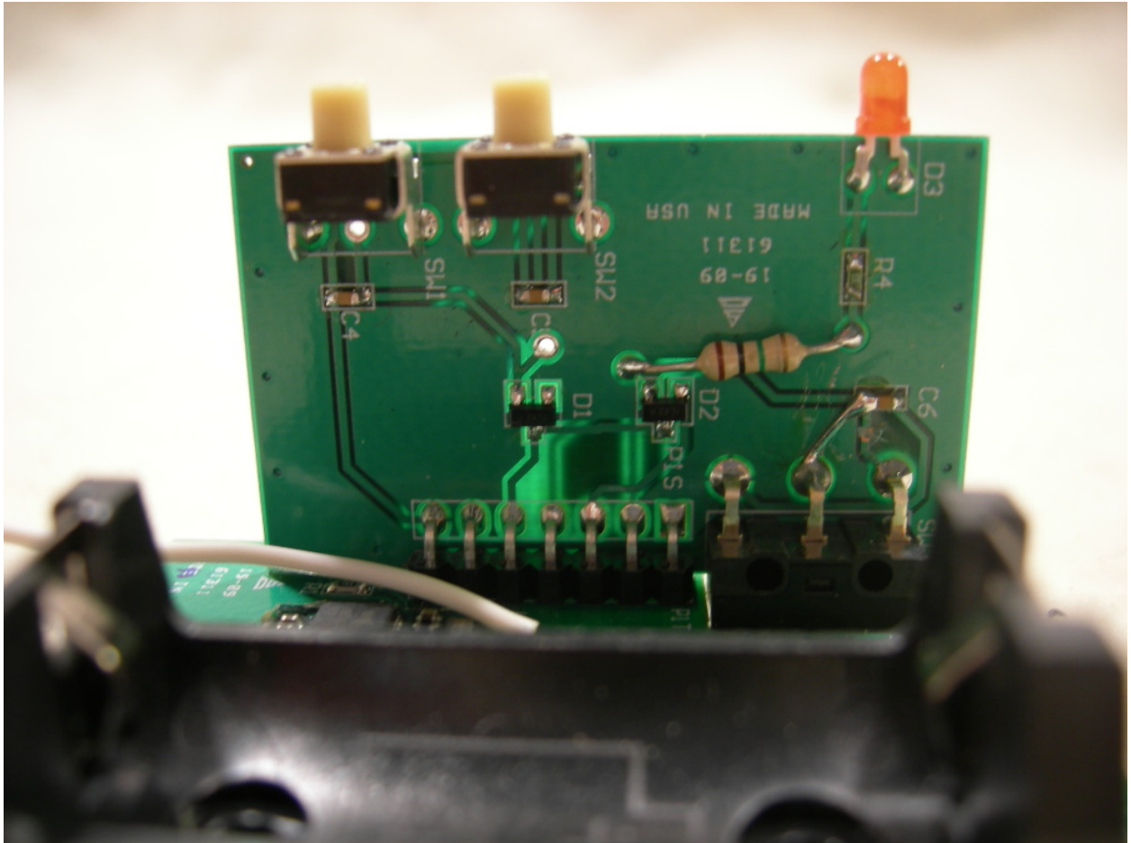
Figure 3: Secondary PCB Front
