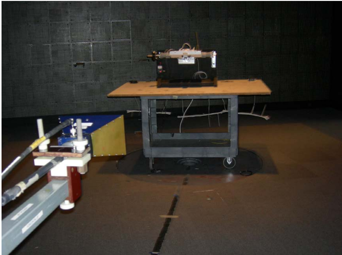
Figure 1: Radiated Emissions
