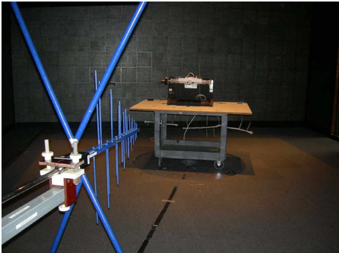
Figure 3: Radiated Emissions
