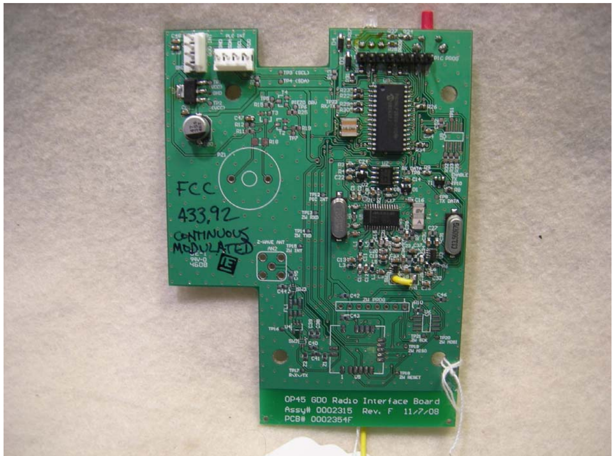
Figure 2: RF PCB - Front
