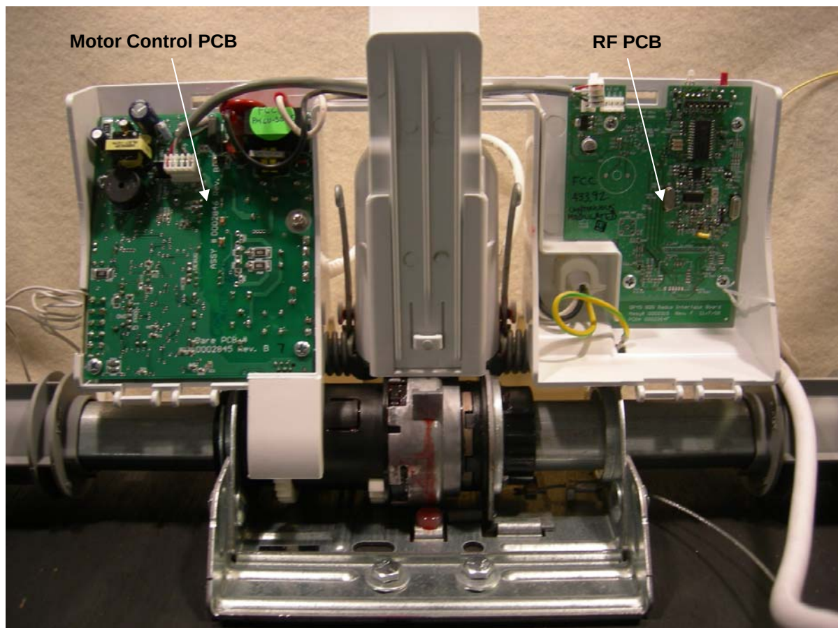
Figure 1: Assembled View (Bottom)
