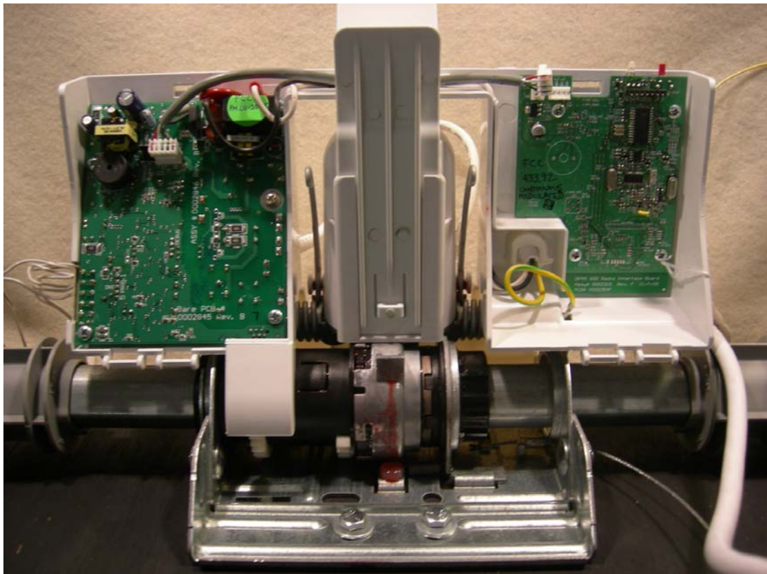
Figure 4: Bottom View Without Cover
