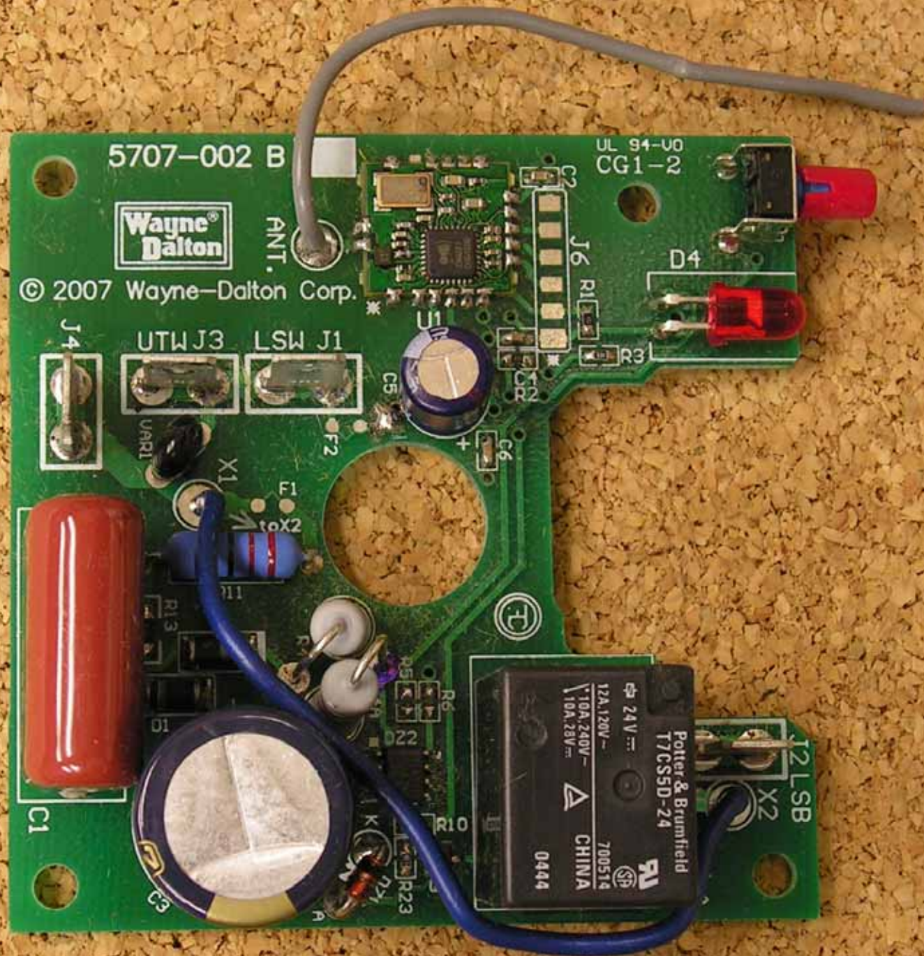
PCB (top)
