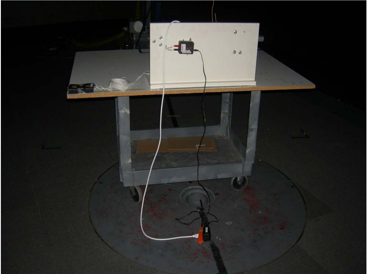
Figure 5: Radiated Emissions – Unintentional
