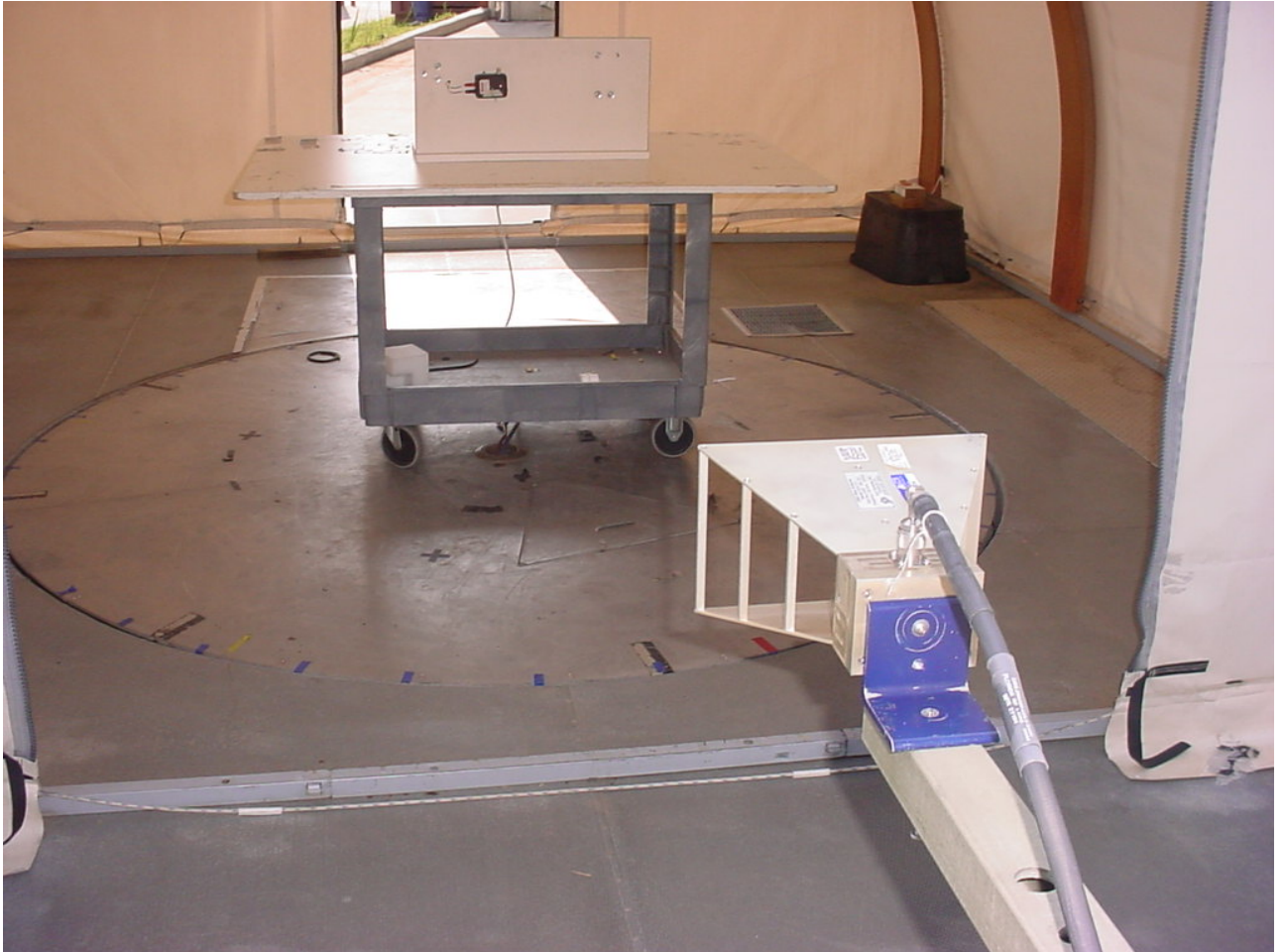
Figure 2: Radiated Emissions – Intentional
