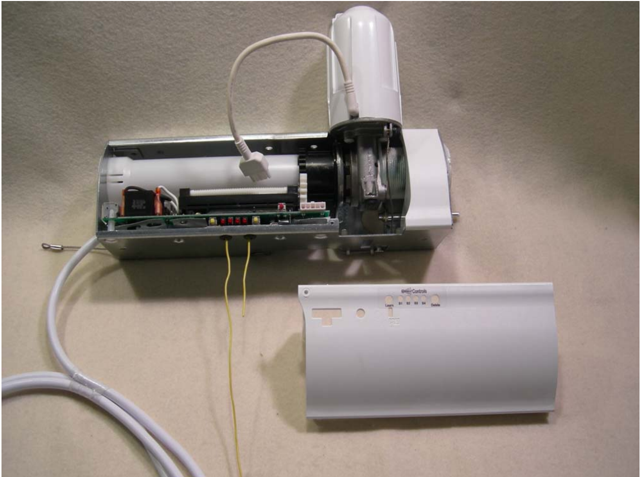
Figure 7: PCB's in garage door motor assembly
