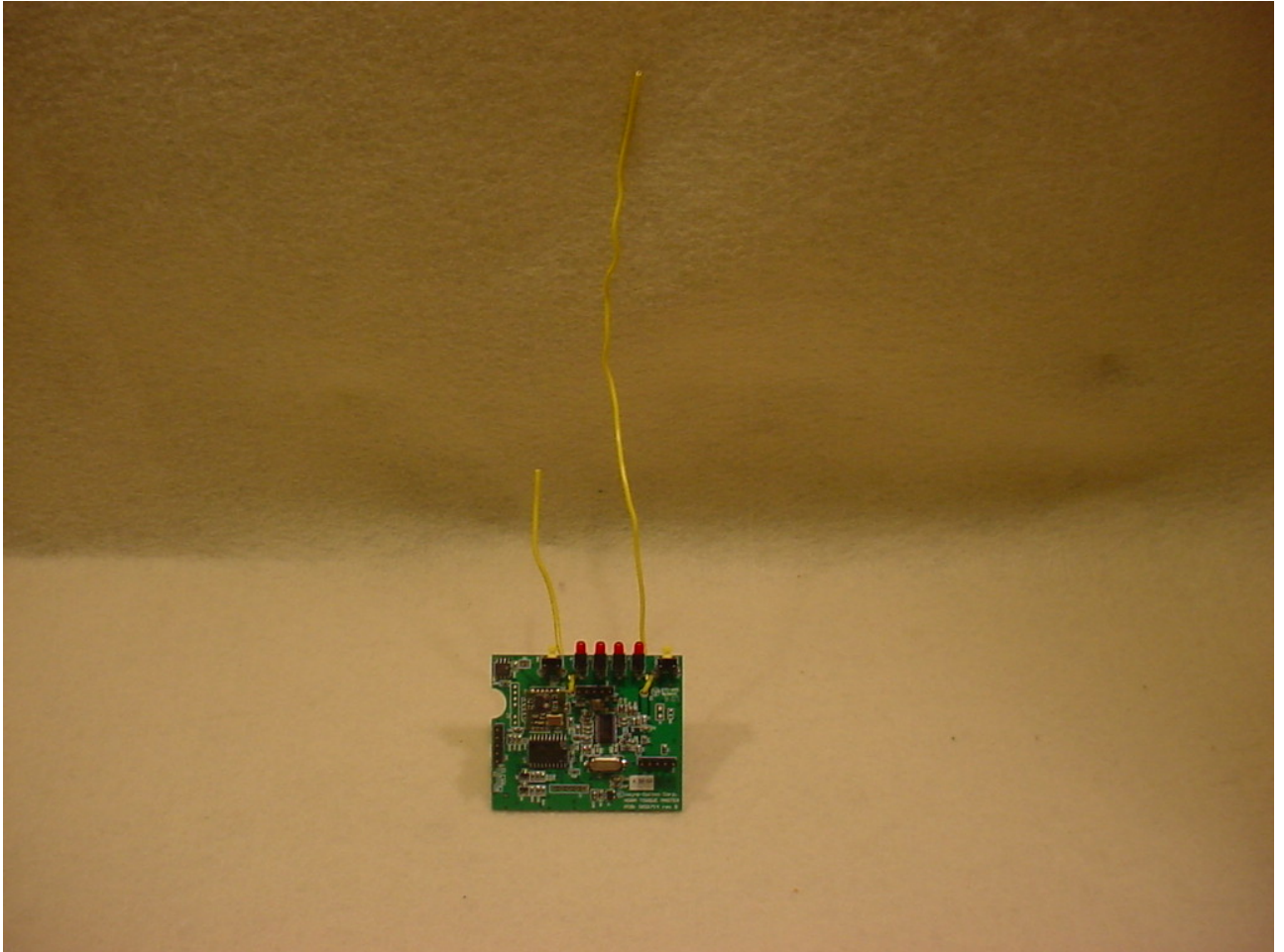
Figure 3: 908.42MHz Transceiver / 372MHz Receiver Board
