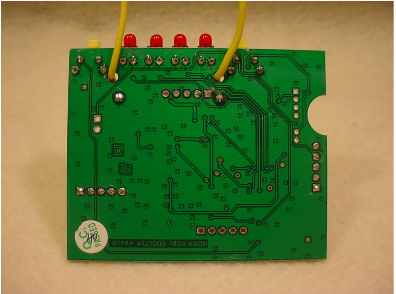
Figure 2: 908.42MHz Transceiver / 372MHz Receiver Board - Back
