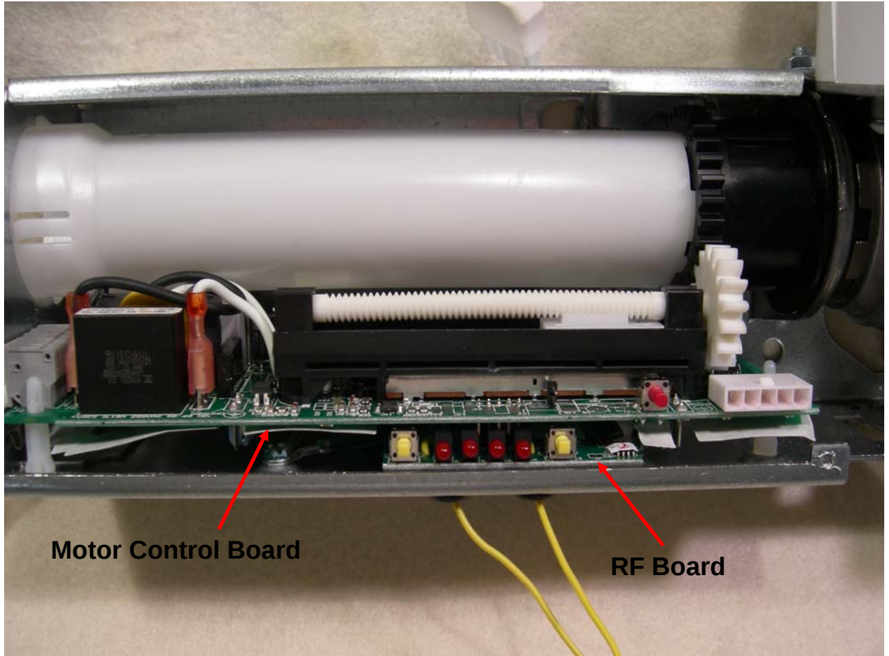
Figure 8: PCB's in garage door motor assembly
