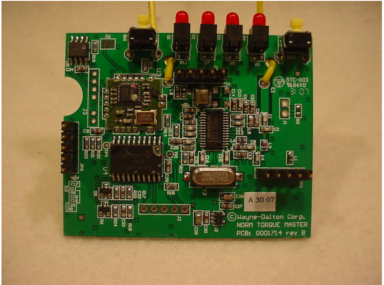
Figure 1: 908.42MHz Transceiver / 372MHz Receiver Board - Front
