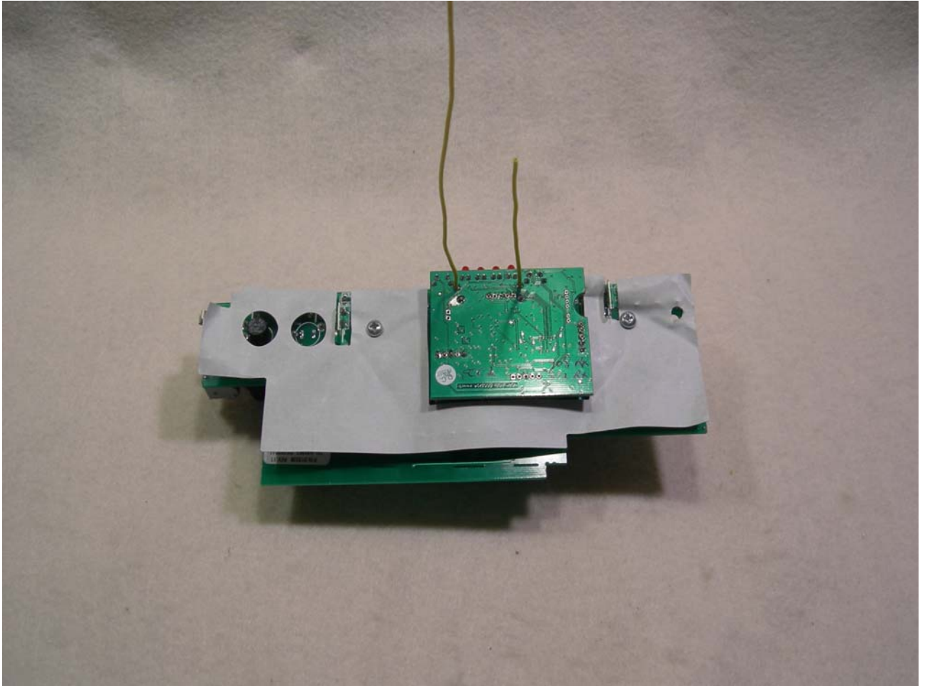
Figure 4: Transceiver / Receiver PCB mounted on Main PCB
