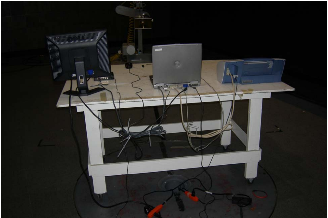
Figure 5: Test Setup Radiated Emissions – Unintentional
