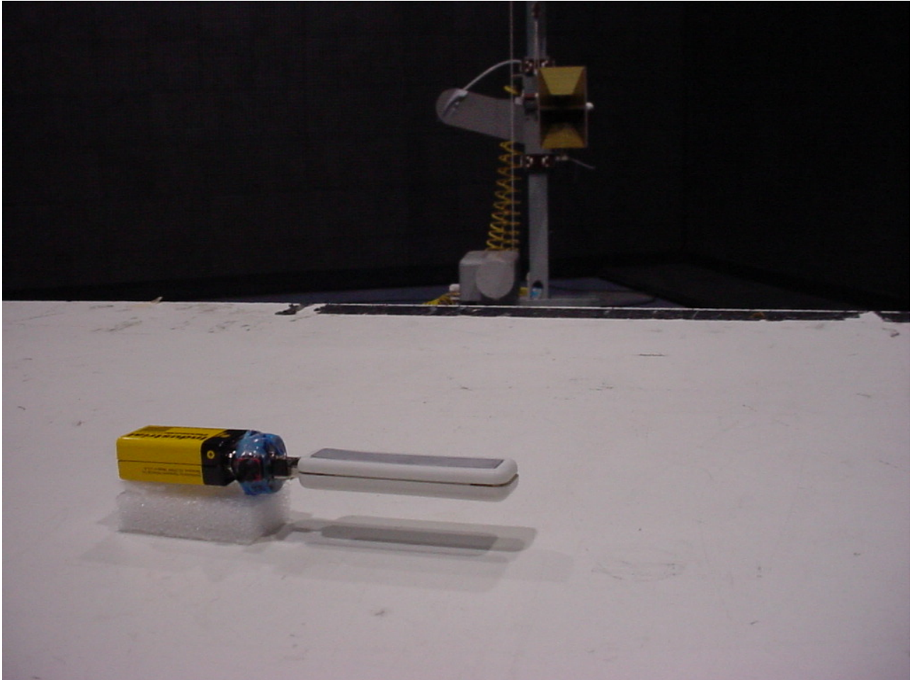
Figure 7: Test Setup Radiated Emissions - Intentional
