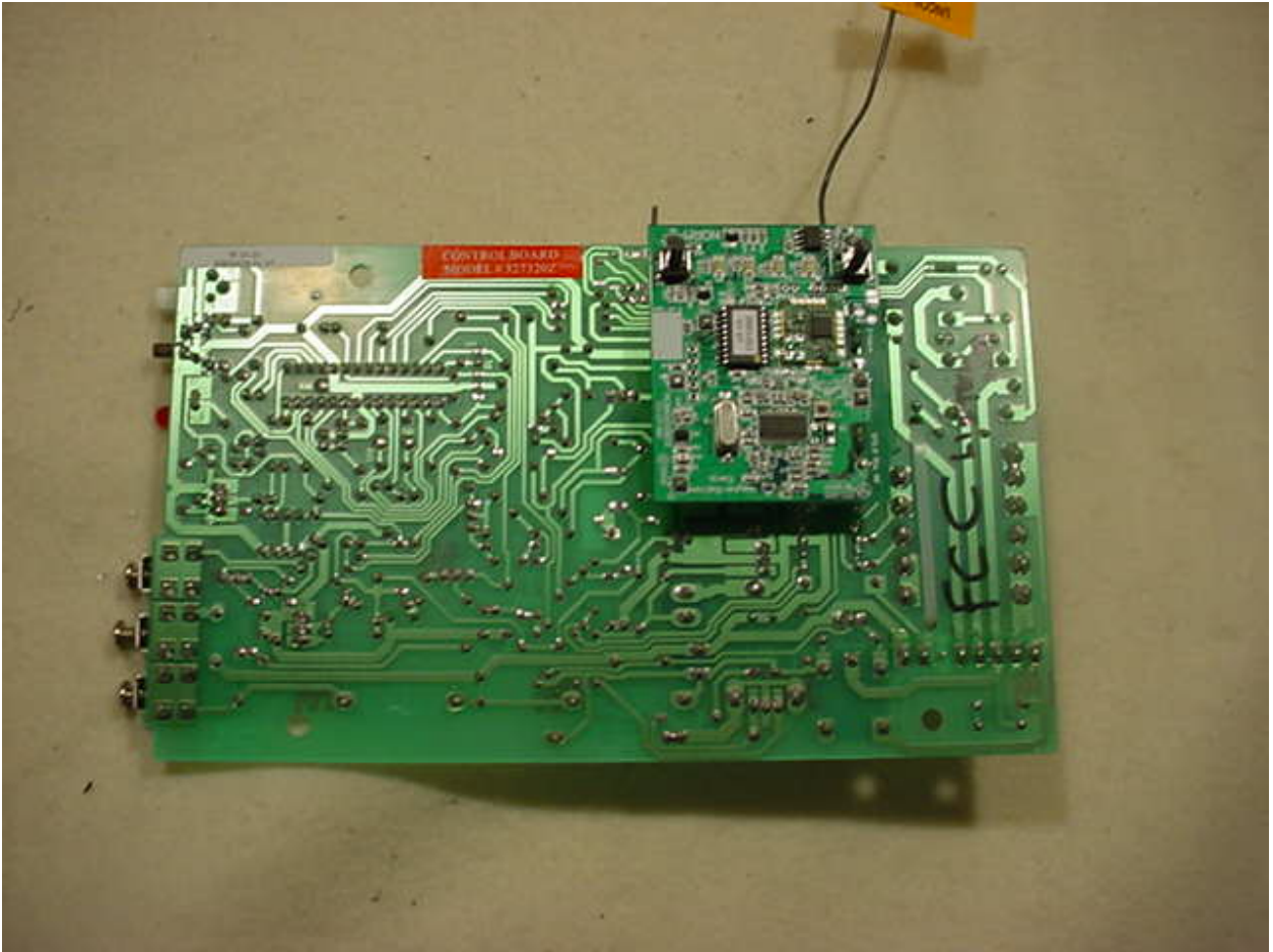
Figure 1: Internal Photographs - Assembled
