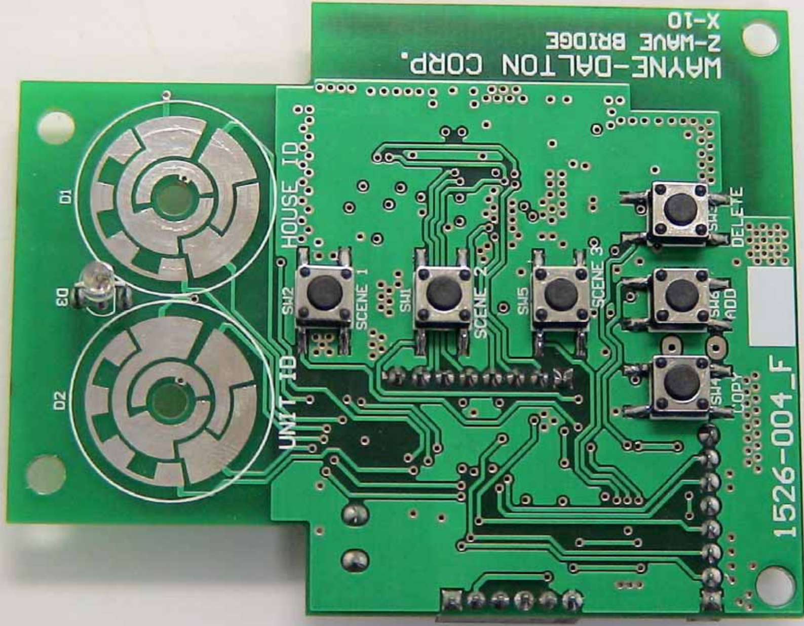
PCB (top)
