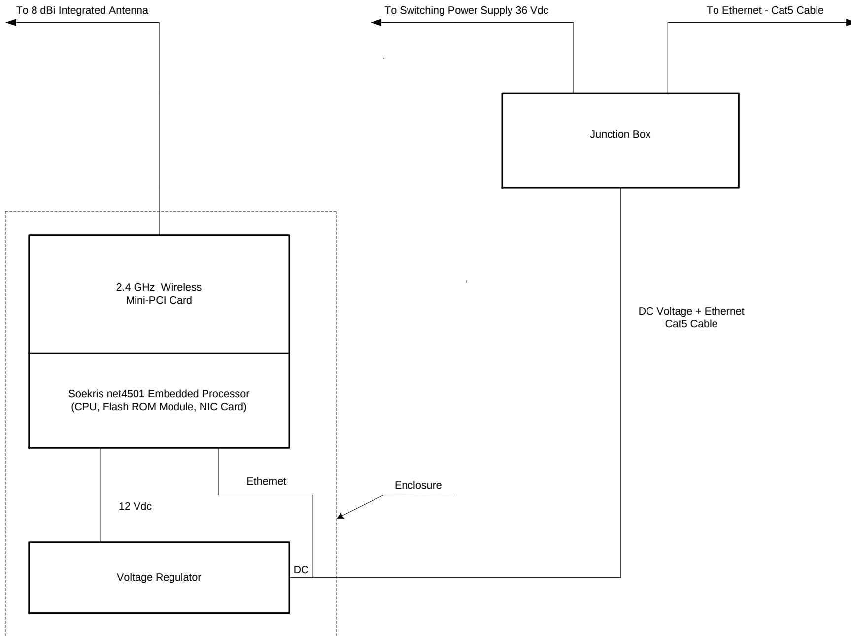
Figure 1. Block Diagram of Wireless Outdoor 2.4 GHz KINSL9201 Router
