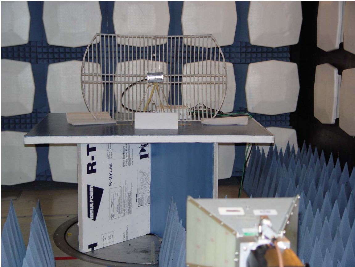
2.4 GHz 24dBi Parabolic
