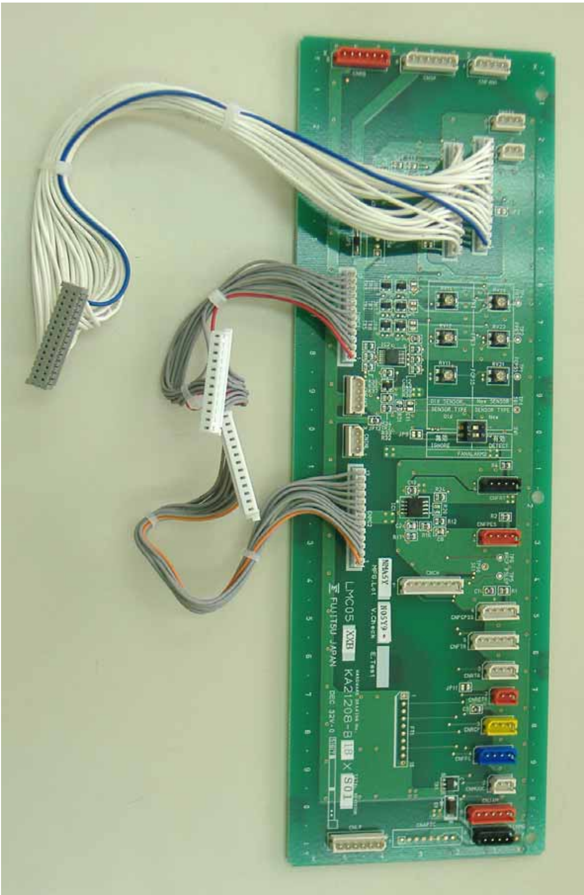
Connector board
