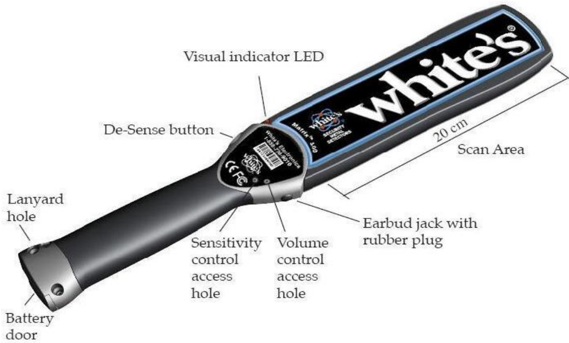
WHITE'S ELECTRONICS MATRIX 100 HANDHELD SECURITY METAL DETECTOR REAR VIEW
