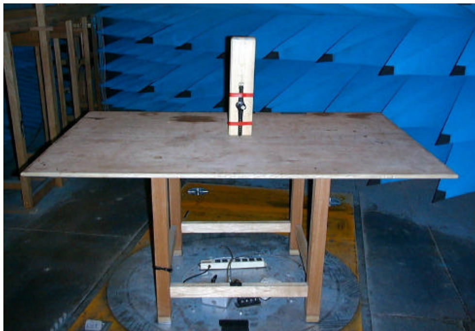
fig 1. Test Configuration of the Radiated Emissions (Front View)
