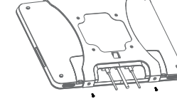
Fasten the set screw to secure the bracket and I/O cover
