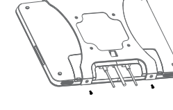
Fasten the set screw to secure the bracket and I/O cover
