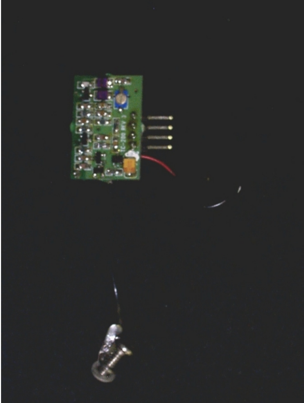
Photo 8. Bottom View of Receiver Board Plus Cable Assembly
