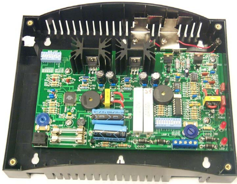
Photo 3. Top View of EUT
