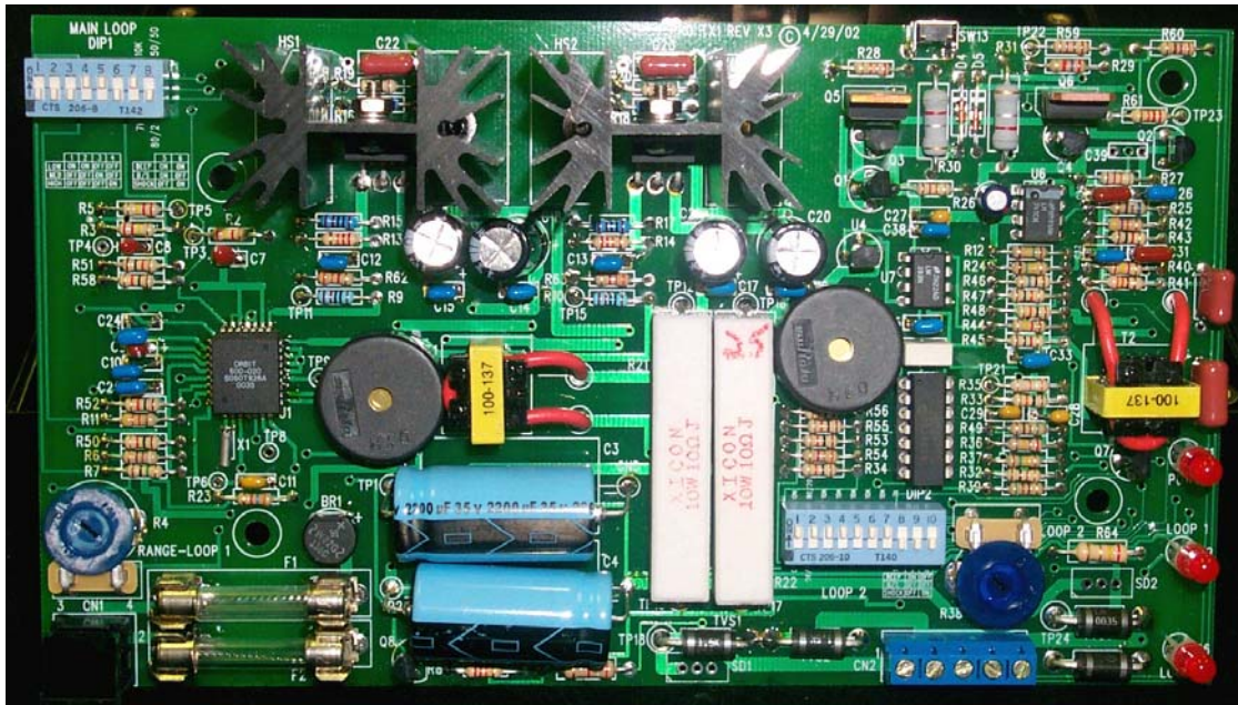
Photo 6. Main Board of EUT, PCB Side
