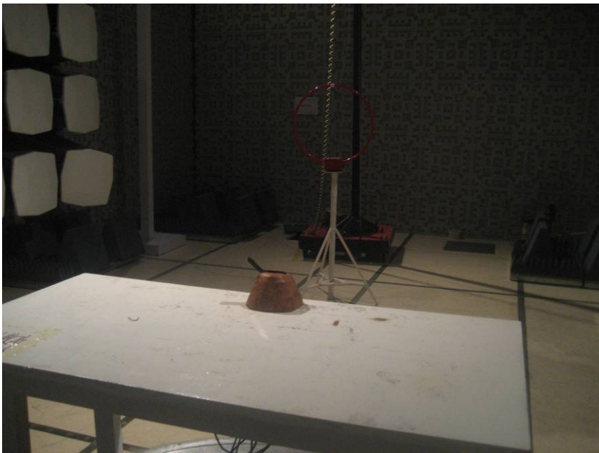
TEST SETUP OF RADIATED EMISSION ( \leq 30 MHz Loop Antenna)
