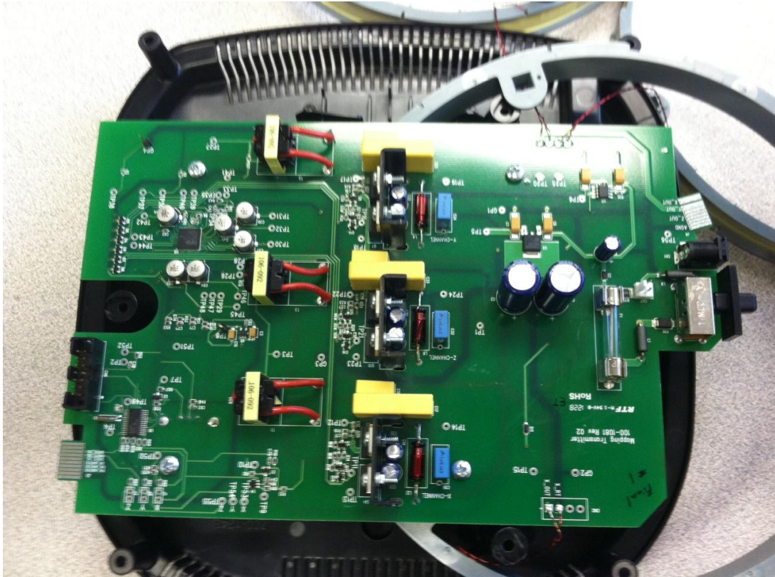
EUT PCB, Component Side
