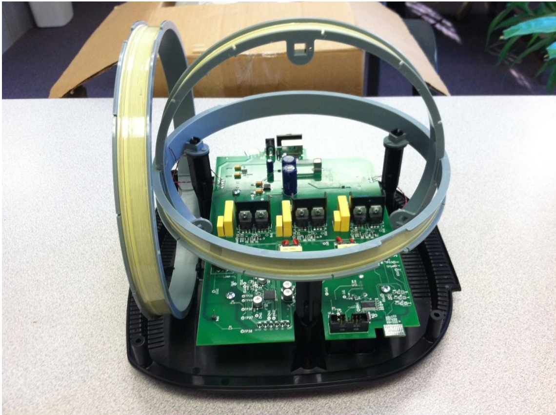
EUT Enclosure Open, Side View
