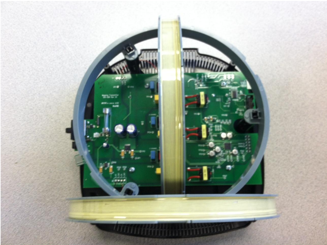
EUT Enclosure Open, Top View
