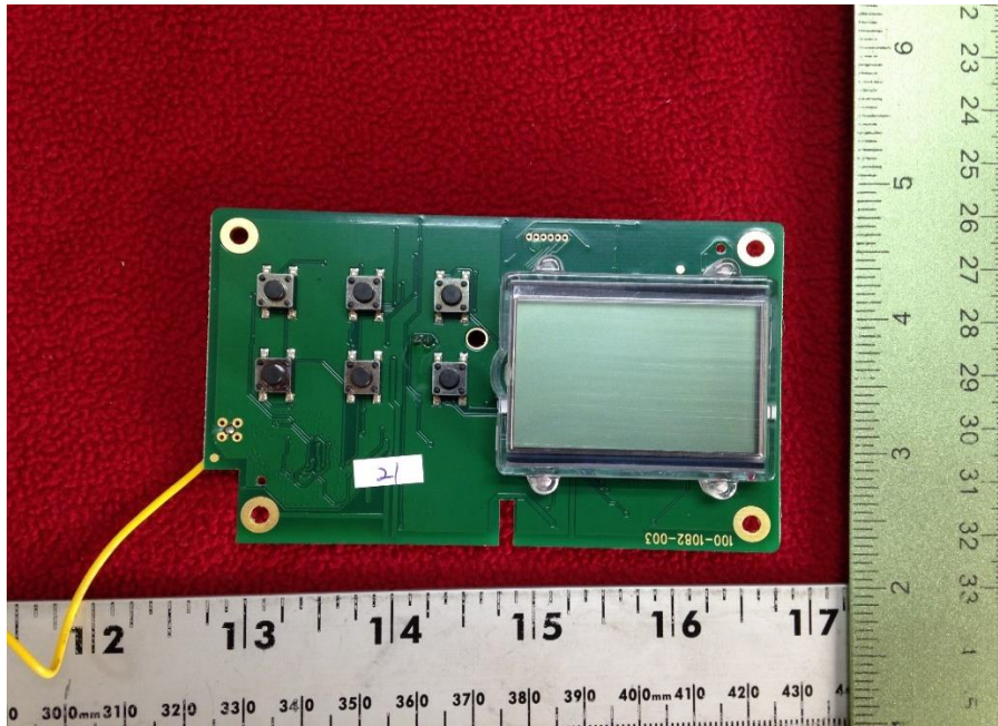
Figure 5. PCB Display Side
