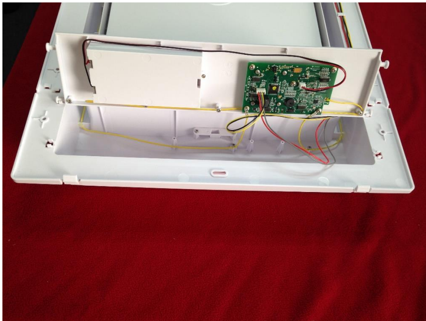
Figure 2. Electronic Module Lifted
