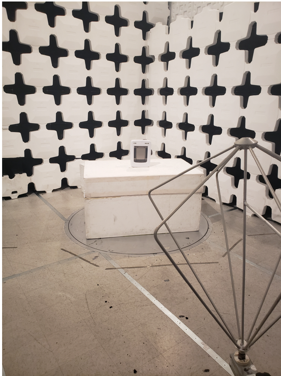
Figure 3. Radiated Emissions Test Setup, 30 MHz to 200 MHz
