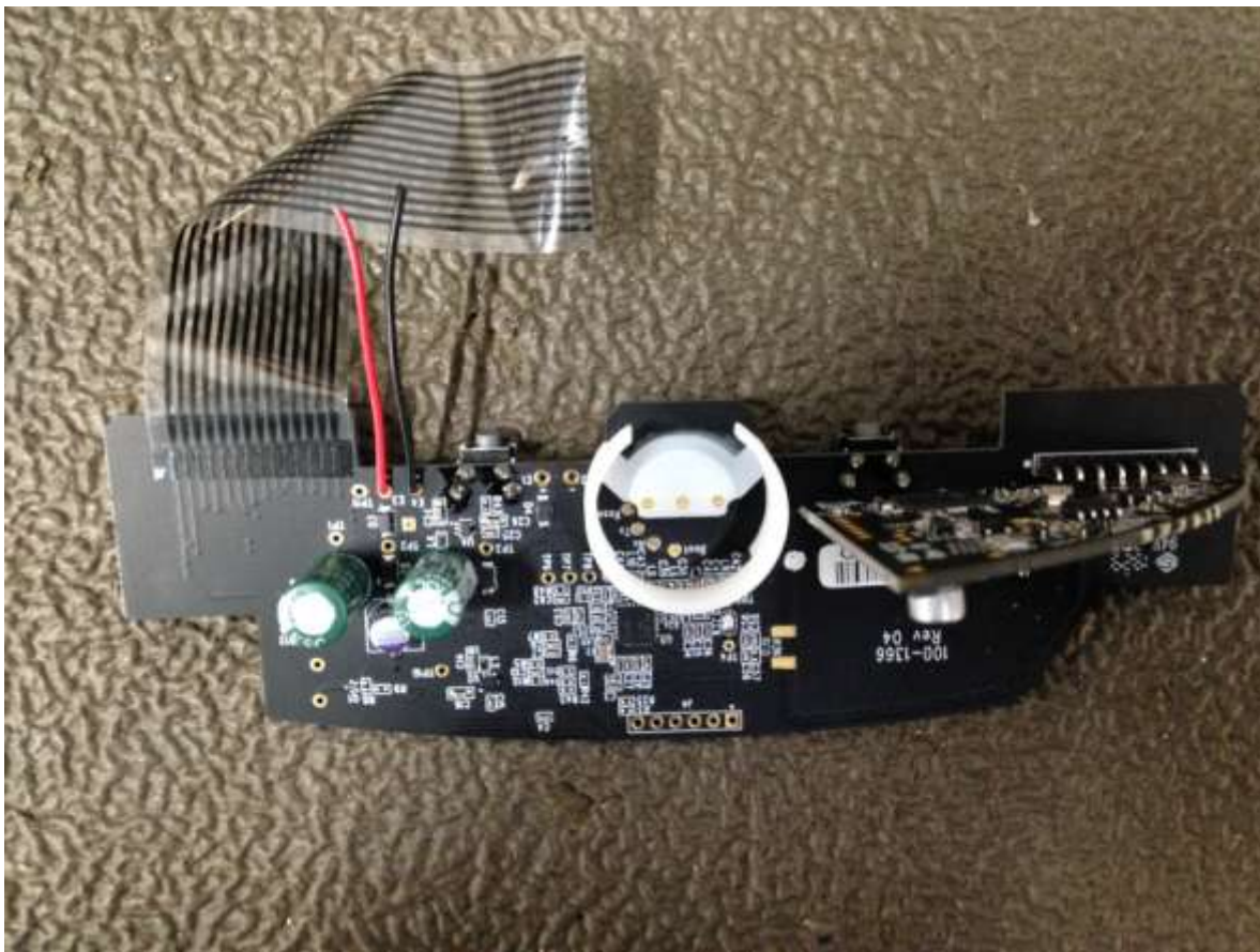
Figure 3. Top of PCB 1, all Models
