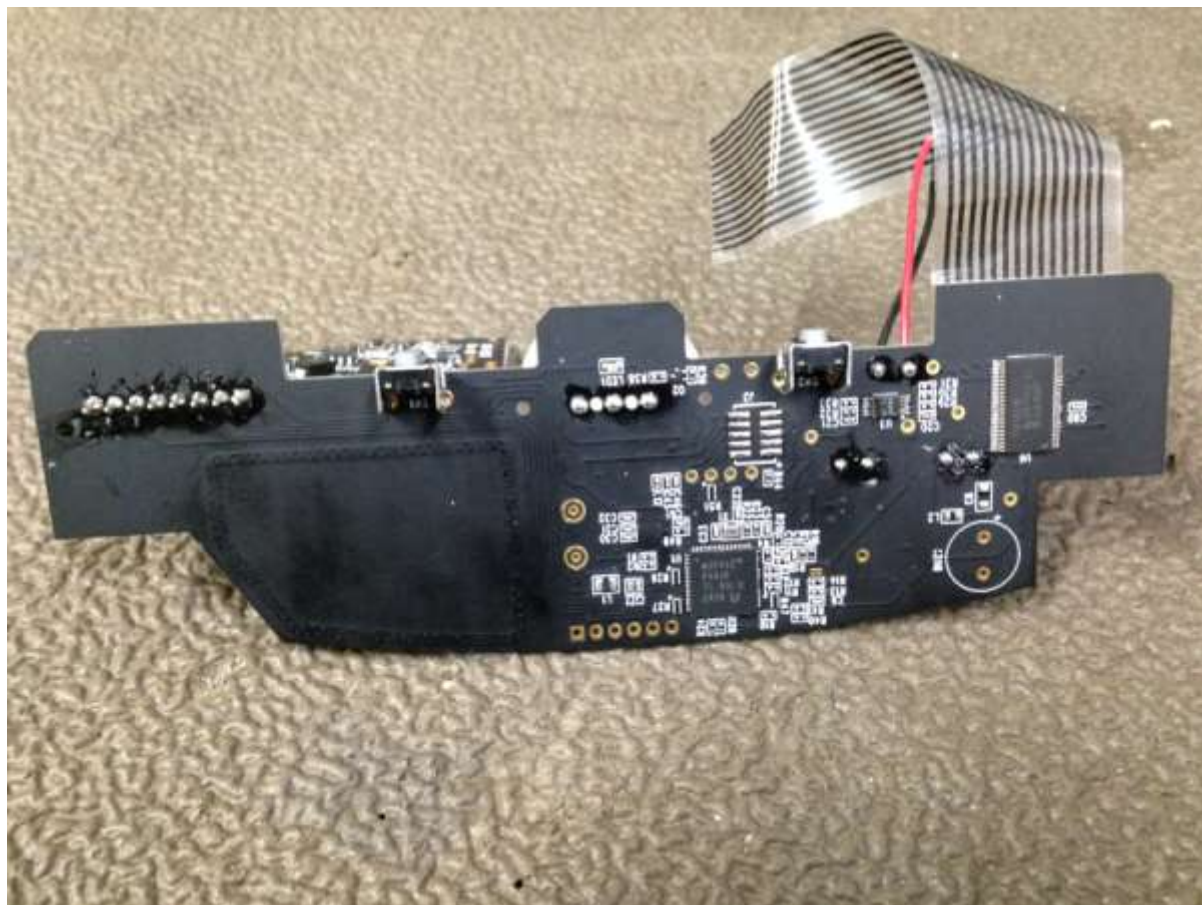
Figure 4. Bottom of PCB 1, all Models
