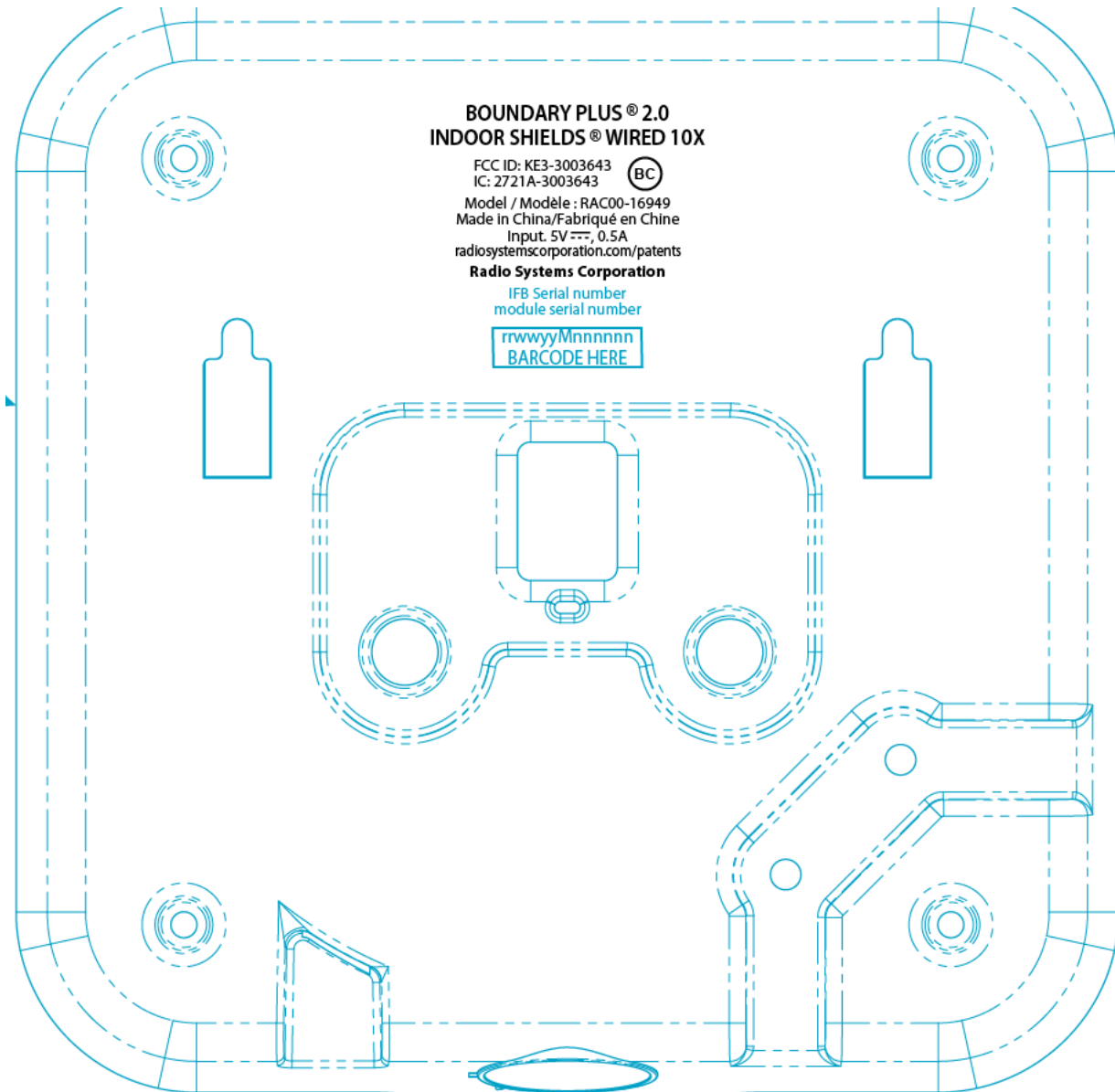
Figure 1. RAC00-16949 Sample Label and Location (Bottom of EUT)
