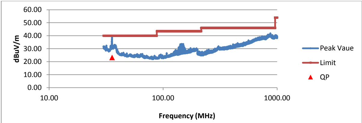
Figure 4. Radiated Emissions Graphical Data, 30 - 1000 MHz – Vertical
