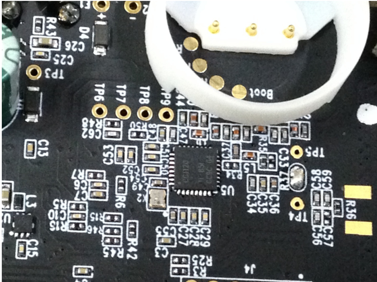
Figure 10. All Models, Close-up of Components Hidden by Plastic Ring
