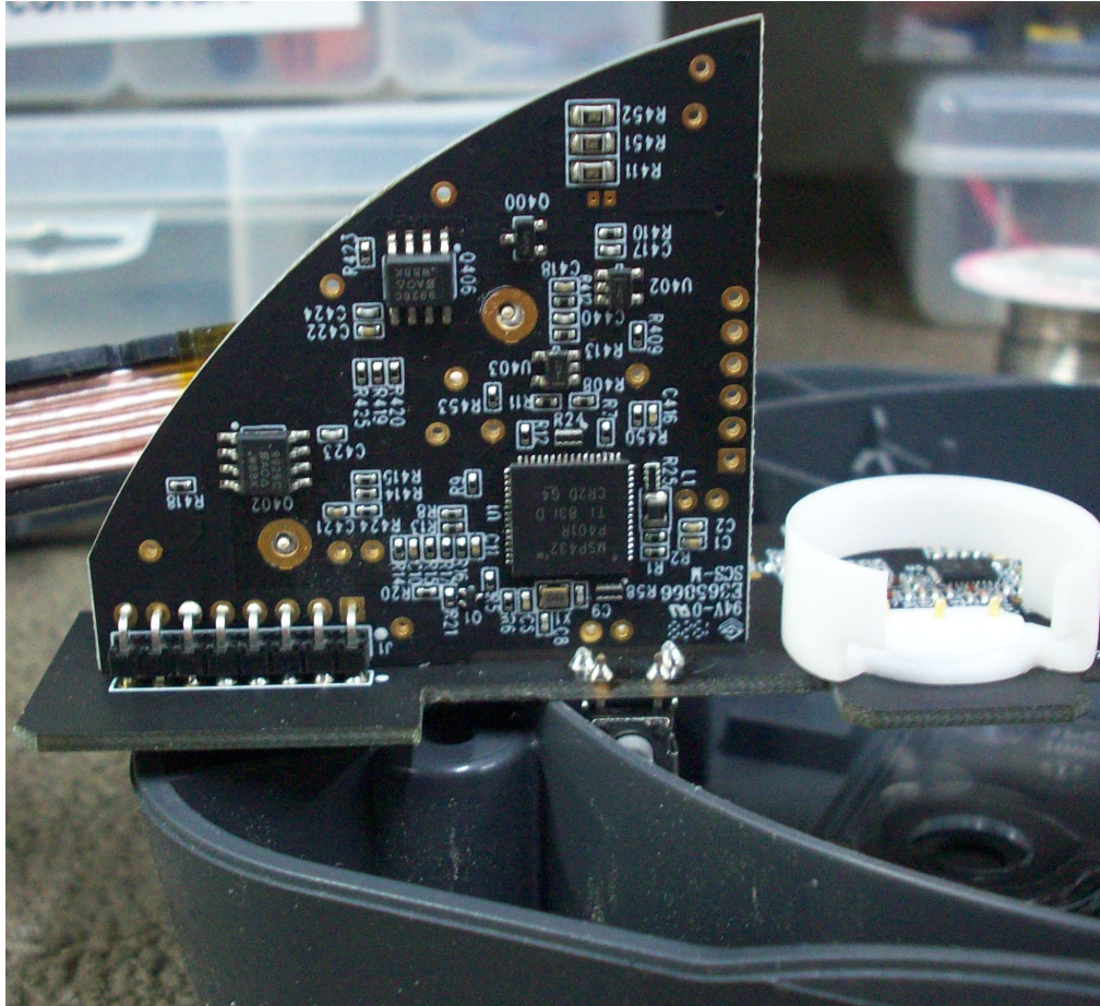
Figure 7. All Models, Bottom of PCB, 1 of 2
