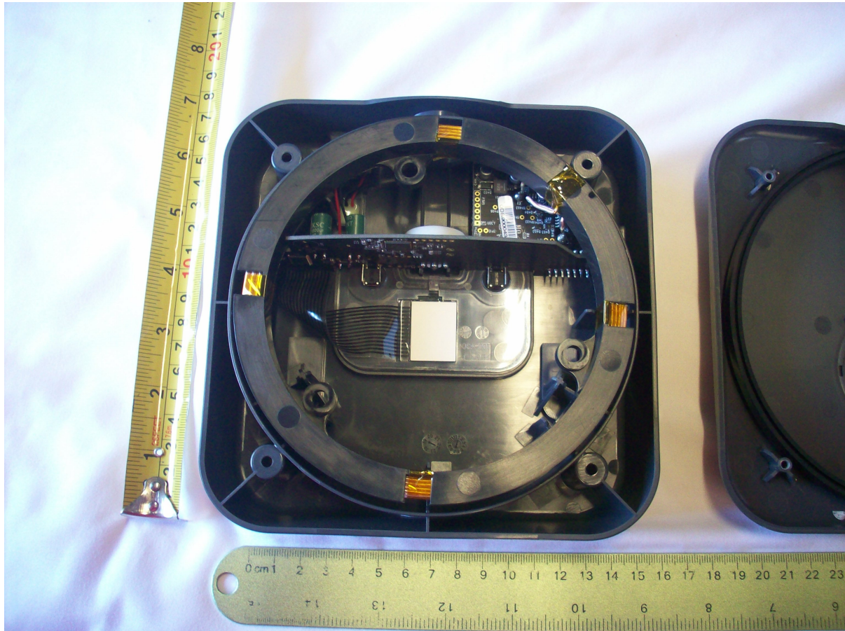
Figure 3. All Models, PCB Close-Up Overview
