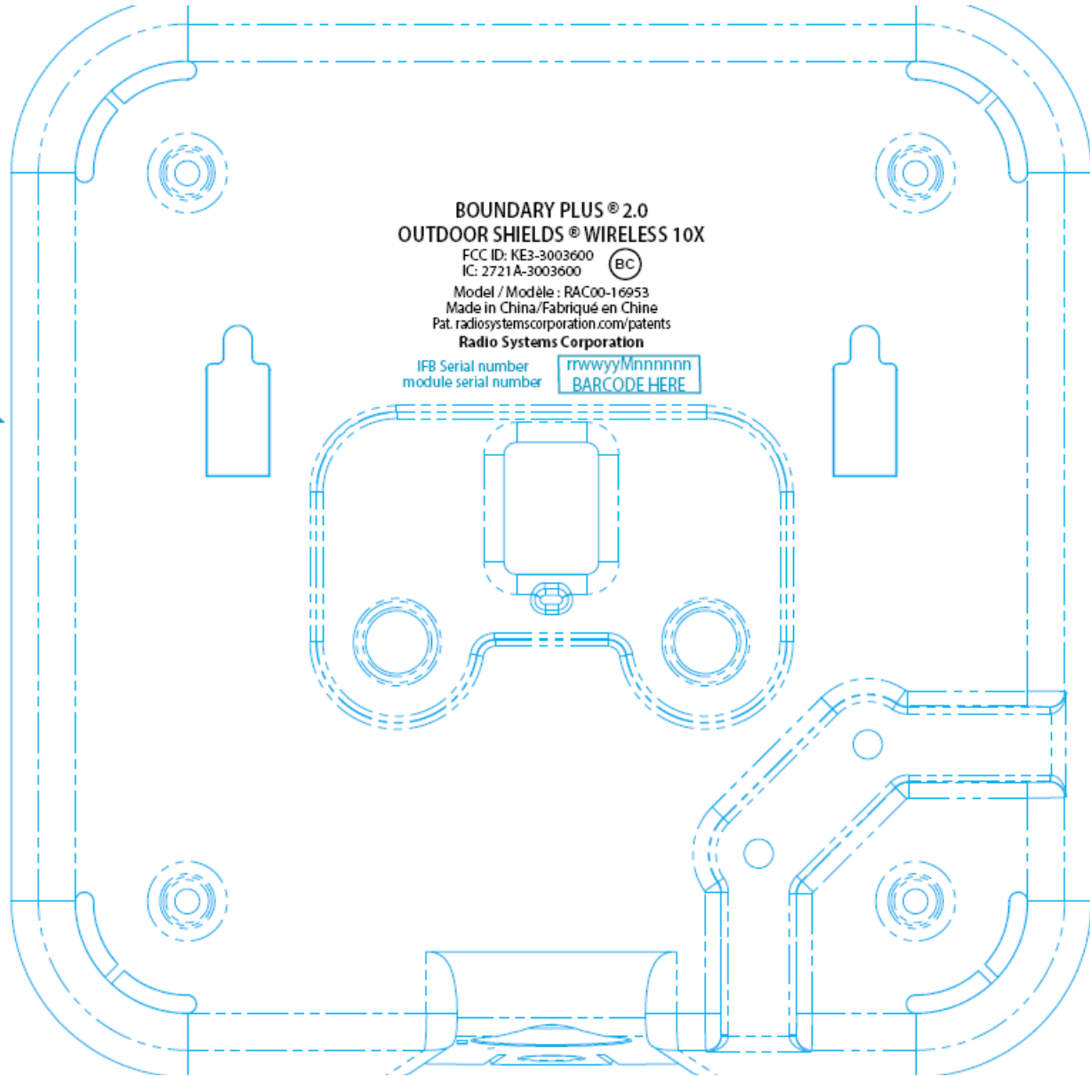
Figure 3. Model RAC00-16953 Sample Label and Location (Bottom of EUT)
