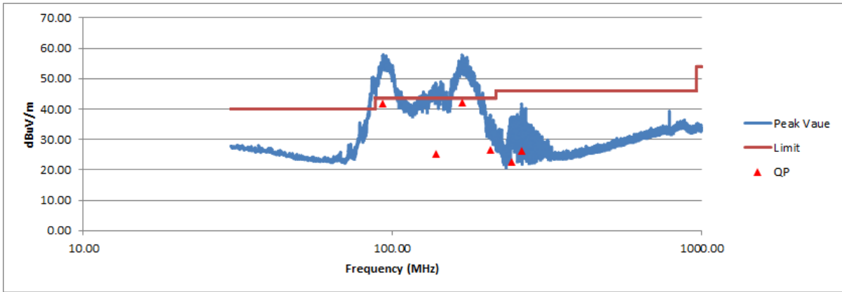
Figure 3. Graphical Data of Radiated Emissions, 30-1000 MHz – Horizontal Position
