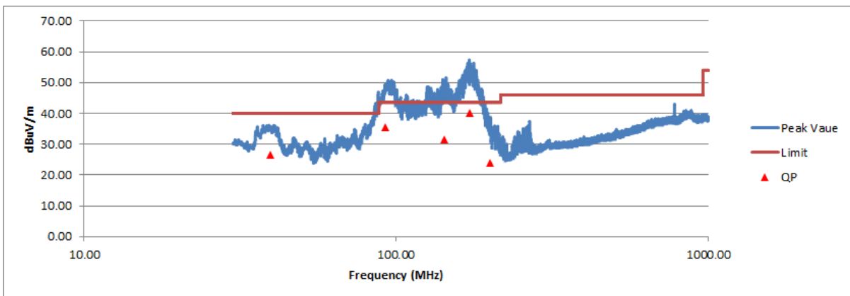
Figure 4. Graphical Data of Radiated Emissions, 30-1000 MHz –Vertical Position
