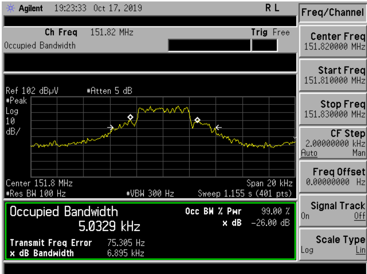
Figure 3. Bandwidth Measurement
