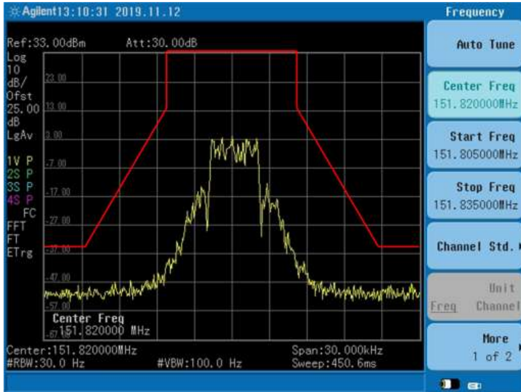
Figure 4. Emission Mask 1
