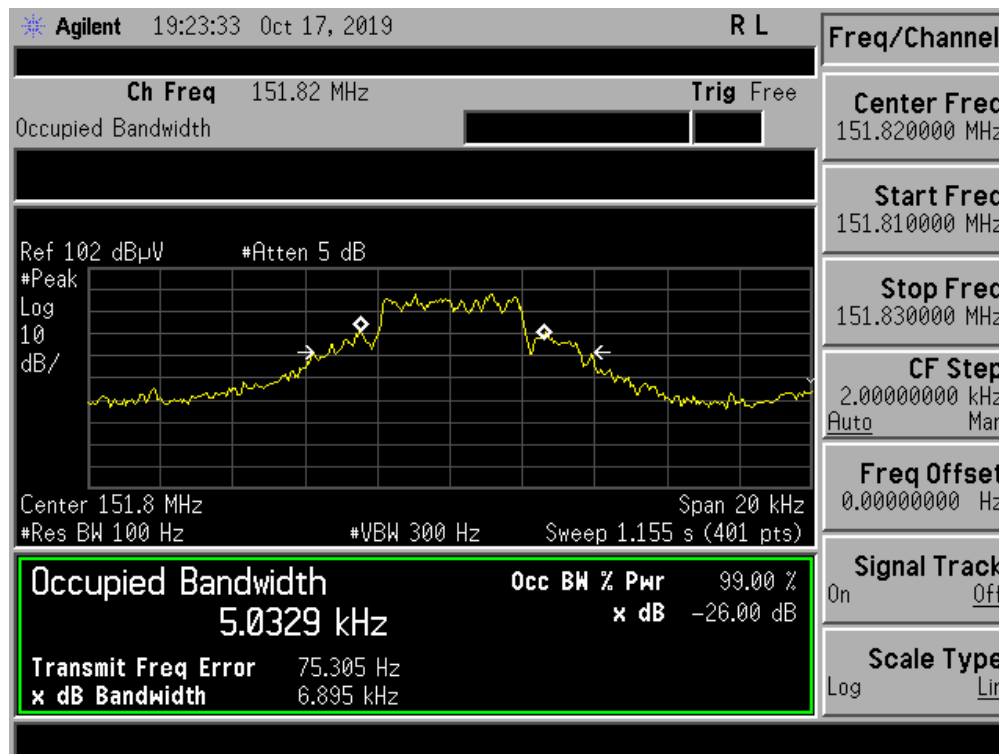
Figure 3. Bandwidth Measurement
