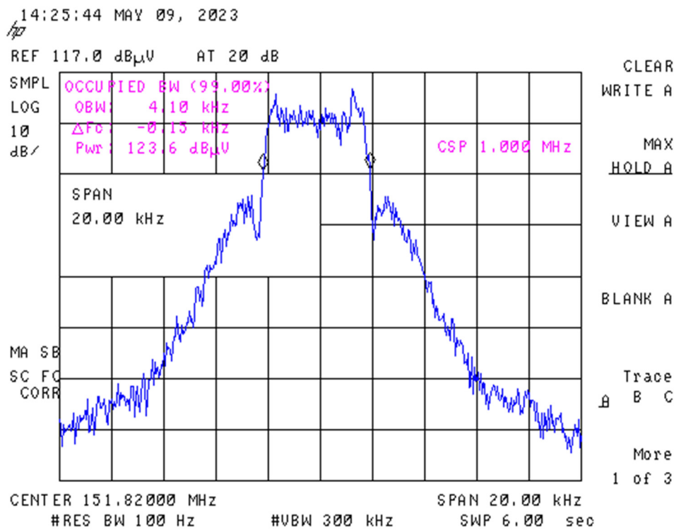
Figure 3. Bandwidth Measurement
