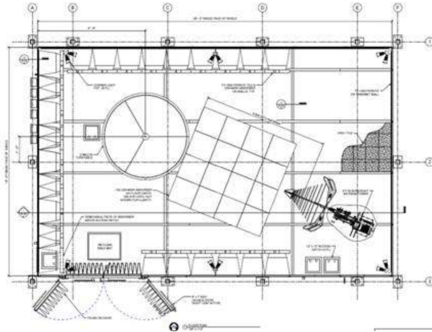
Figure 1. Radiated Emissions Disturbance Measurement Facility Diagram
