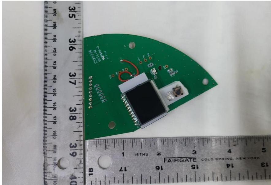
Figure 3. Display Board Front
