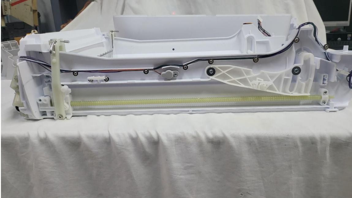
Figure 7. Internal Mechanism Right
