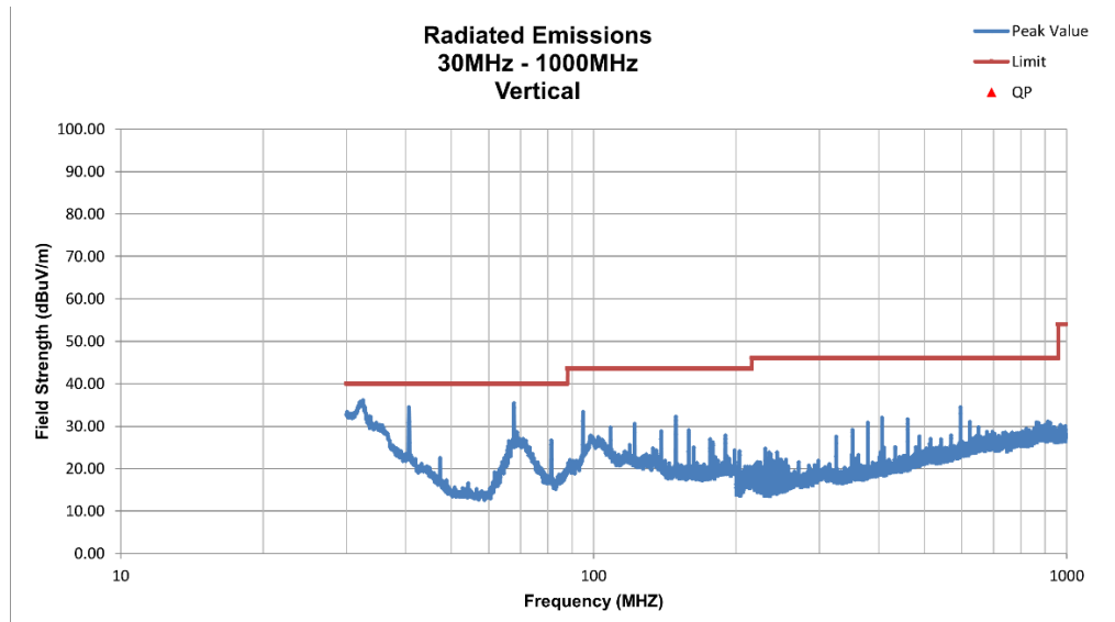
Figure 3. Radiated Emissions 30 - 1000 MHz Vertical
