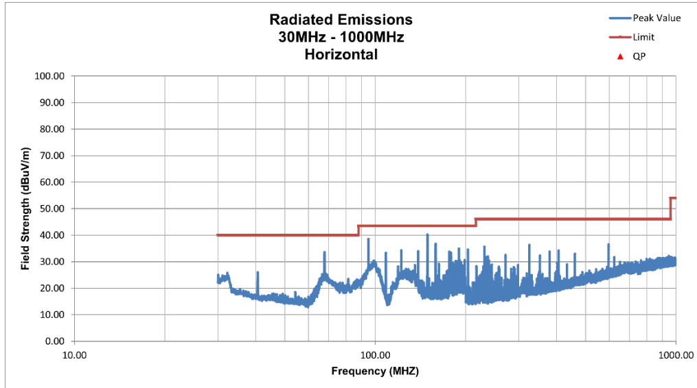
Figure 2. Radiated Emissions 30 - 1000 MHz Horizontal
