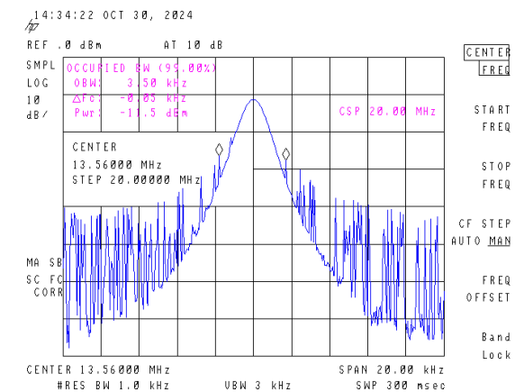
Figure 4. EUT Bandwidth Measurements (20 dB & 99% BW)
