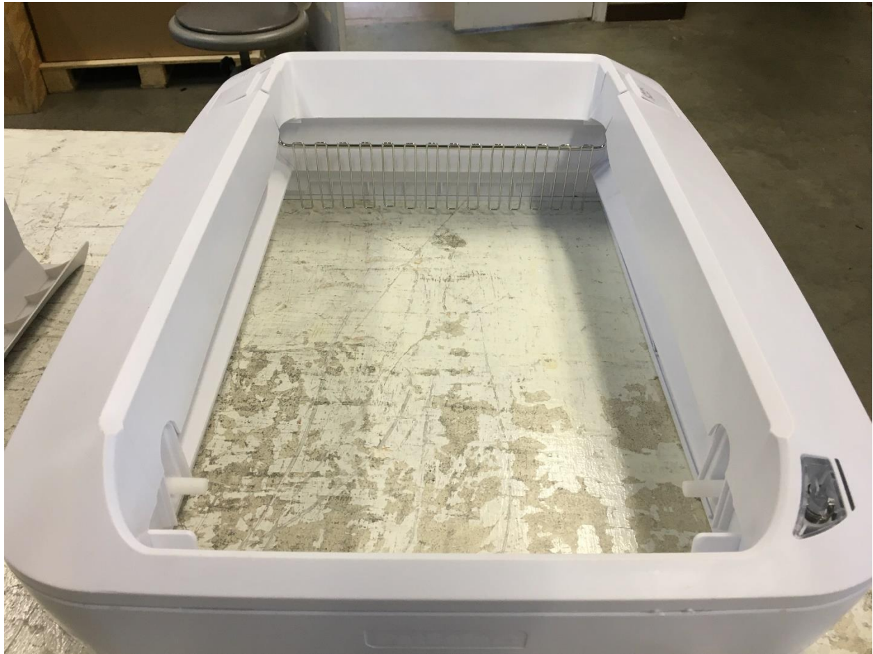
Figure 11. EUT Rake view
