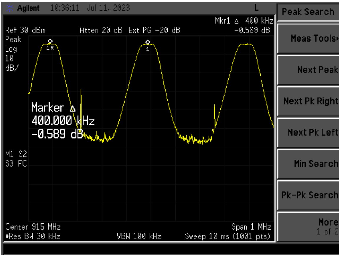
Figure 22. Channel Separation
