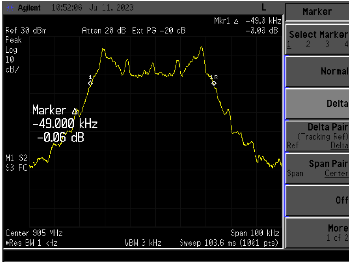
Figure 12. Twenty dB Bandwidth – Low Channel
