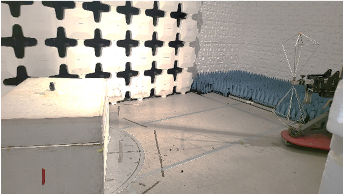
Figure 3. Radiated Emissions Test Setup, 30 MHz to 200 MHz, Back
