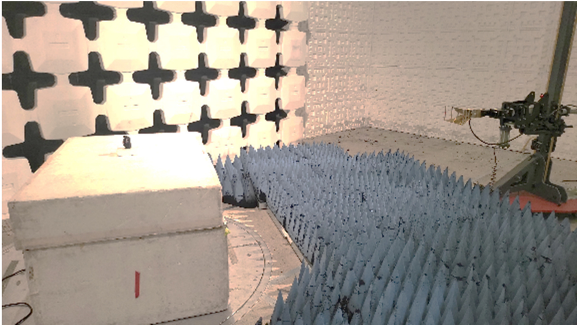
Figure 5. Radiated Emission Test Setup, above 1 GHz, Back
