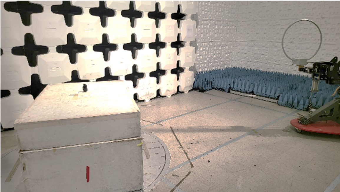
Figure 2. Radiated Emissions Test Setup, 9 kHz to 300 MHz, Back
