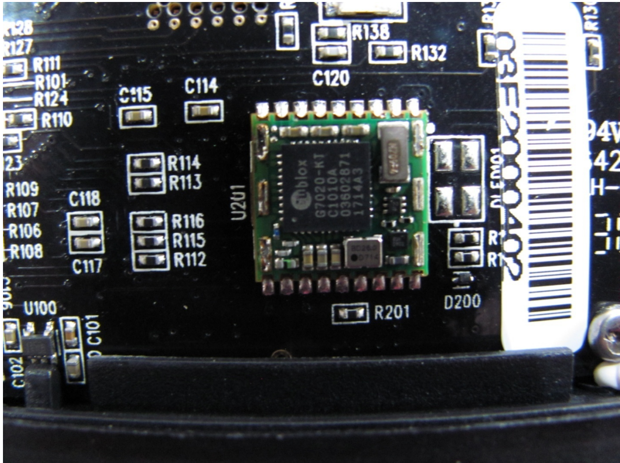
Figure 6. Side 1, Shield Removed
