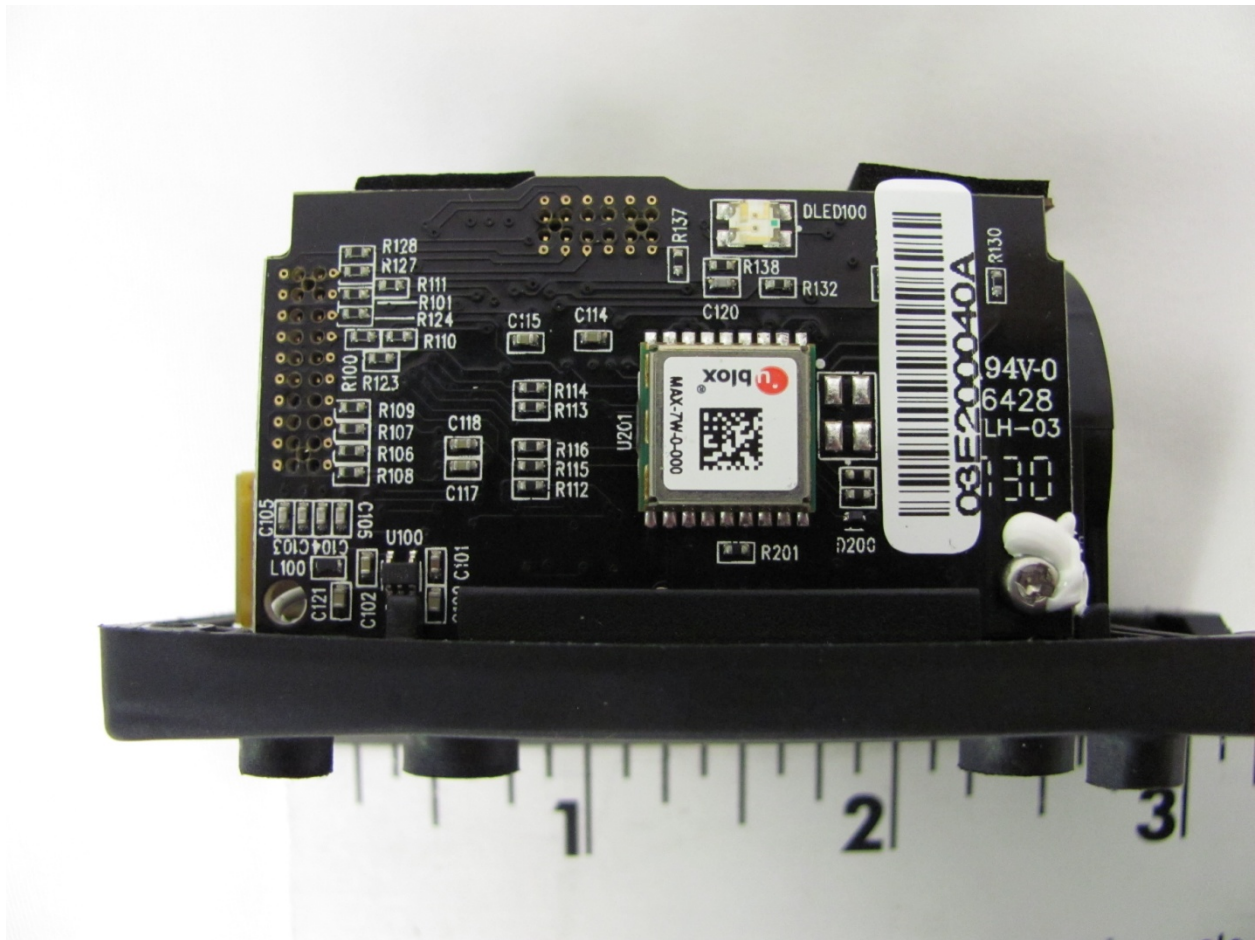
Figure 1. Side 1 (Processor Board and LED)
