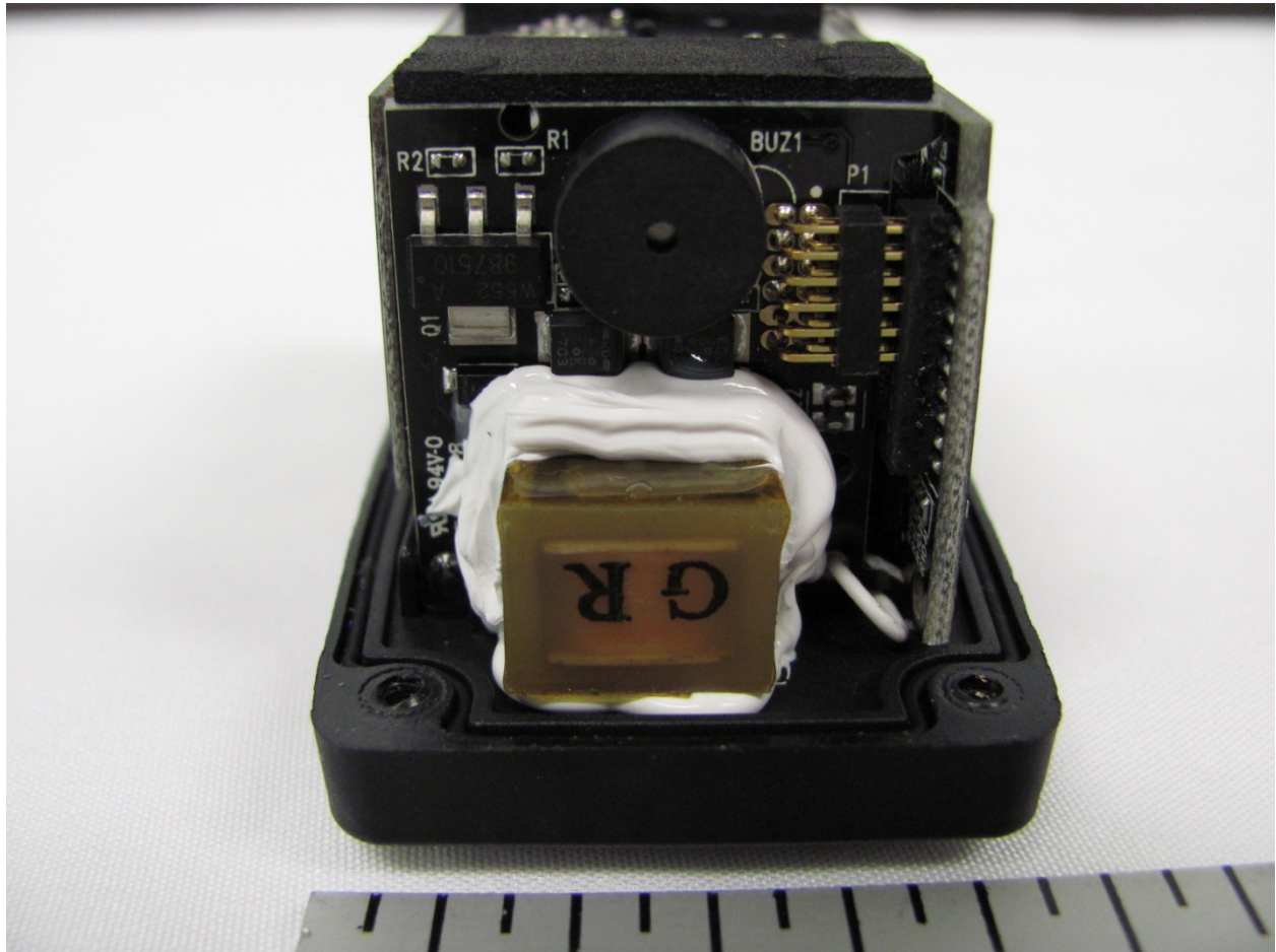
Figure 3. Side 3 (Buzzer)
