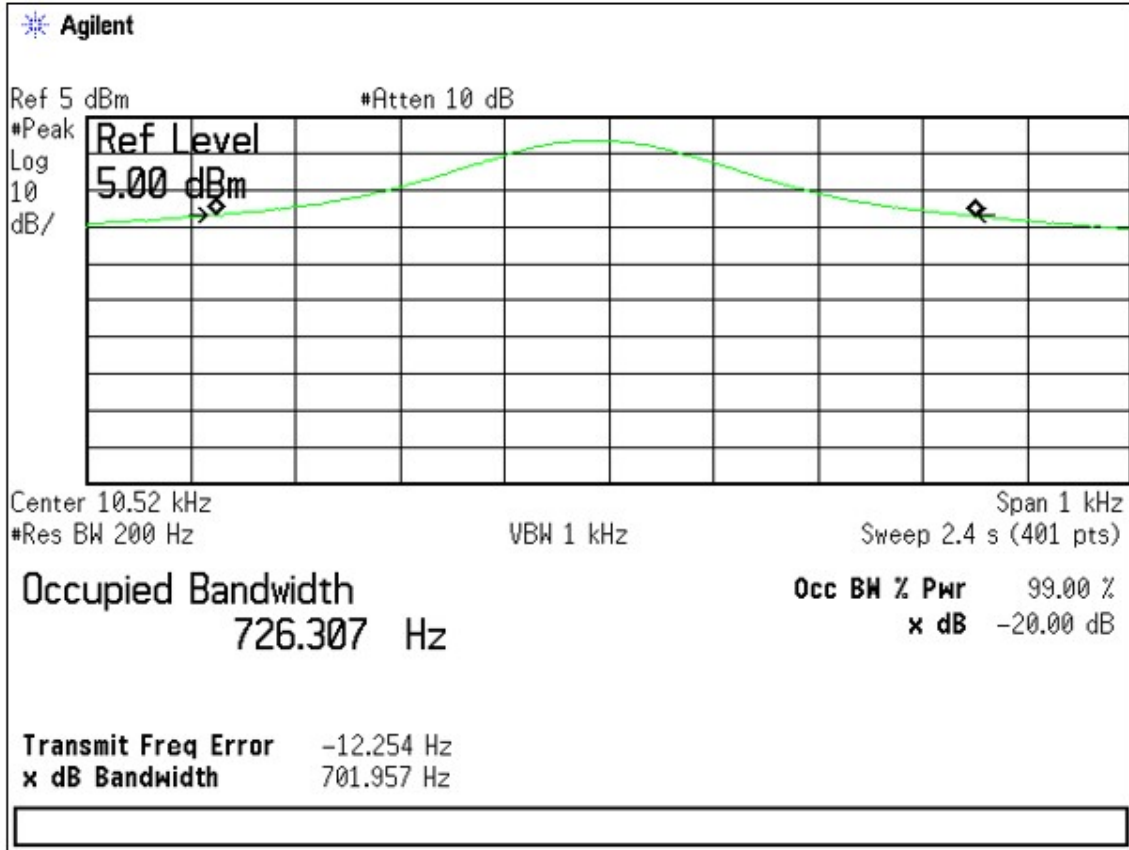
Figure 2. 20 dB & 99% Bandwidth
