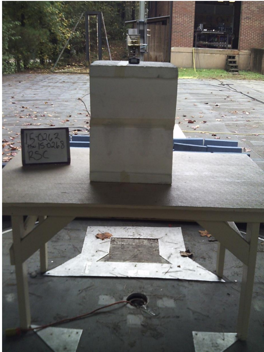
Figure 5. Radiated Emissions Test Setup (Above 1 GHz, Back View)
