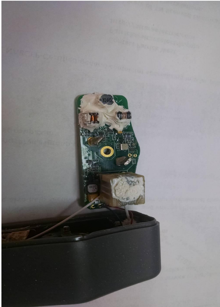
Figure 2. Component Side of PCB
