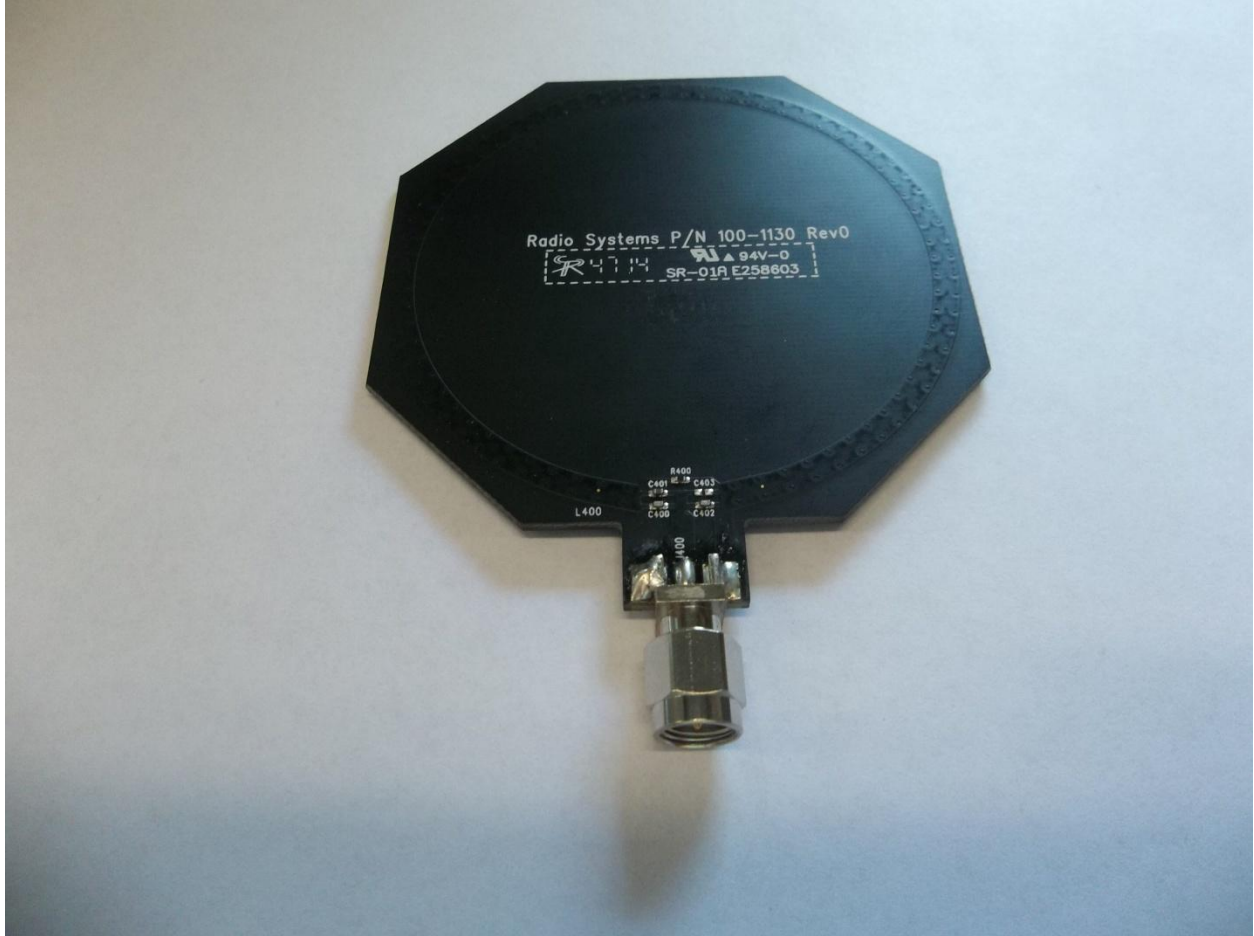
Figure 2. Transmitting Antenna Back
