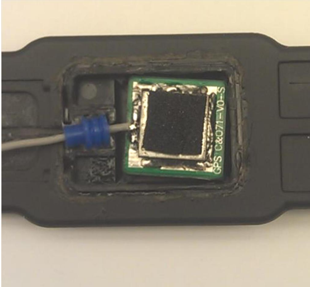
Figure 6. Bondale GPS Antenna
