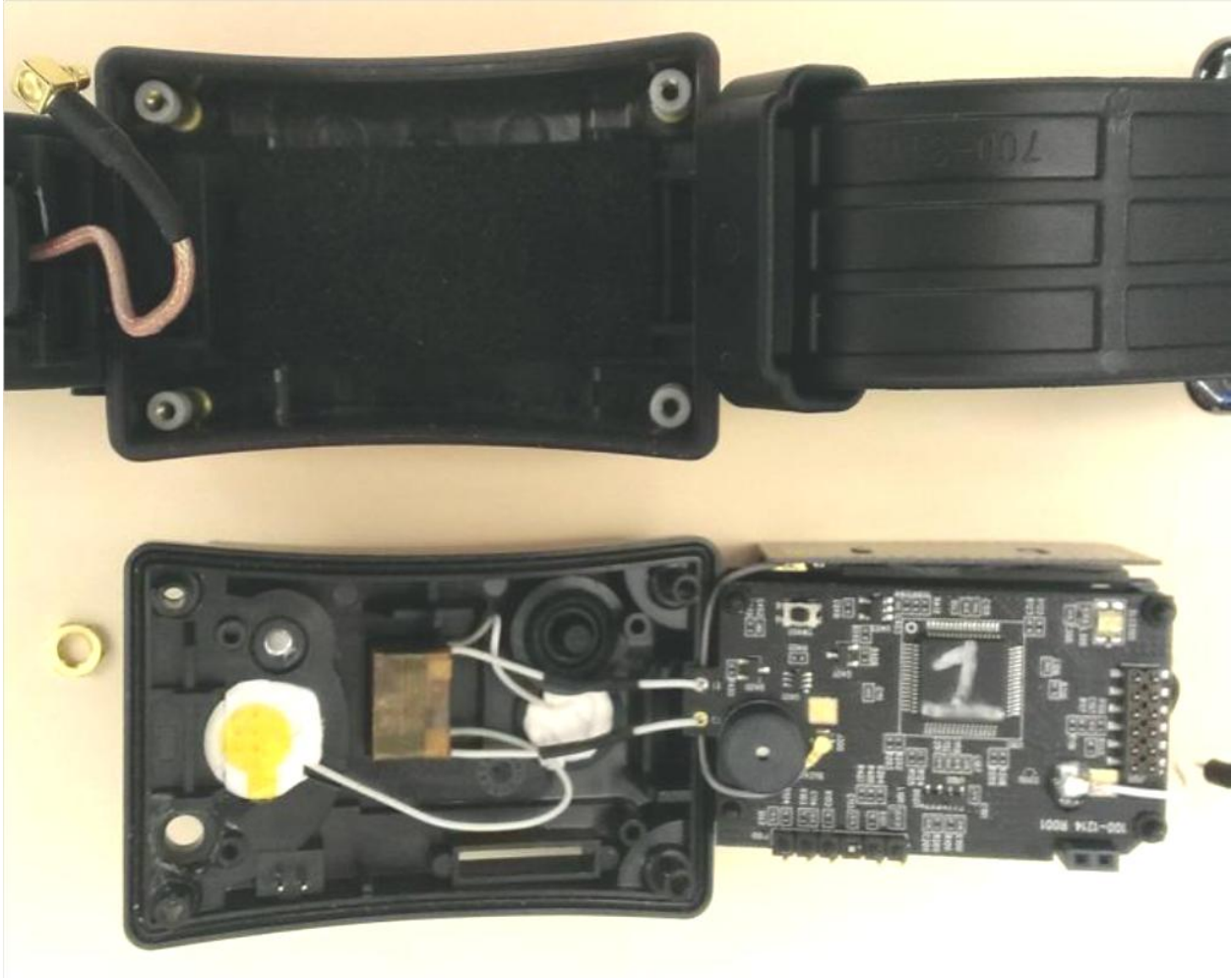
Figure 5. PCBA Mobile Main PCB with transformer
