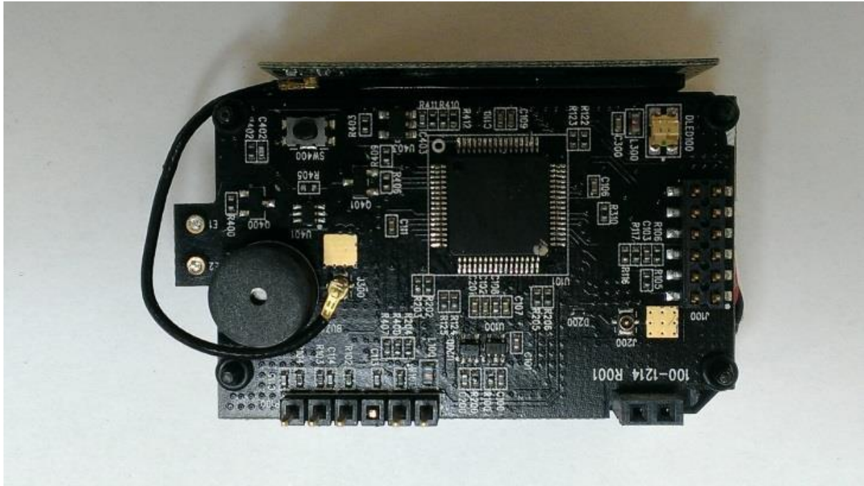
Figure 2. PCBA Mobile 2.0 Main PCB (Bottom)
