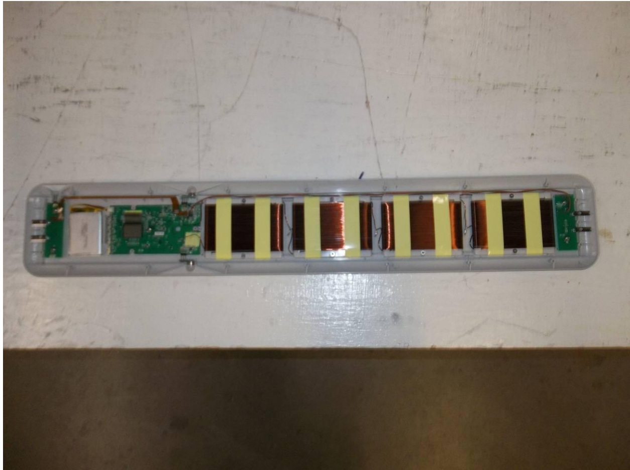
Figure 2. Back of EUT with External Cover Removed
