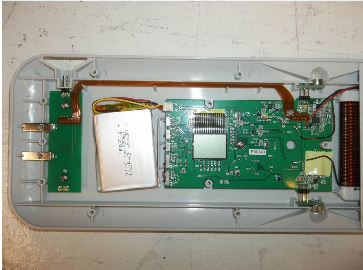
Figure 3. Close Up of EUT with #1 Cover Removed
