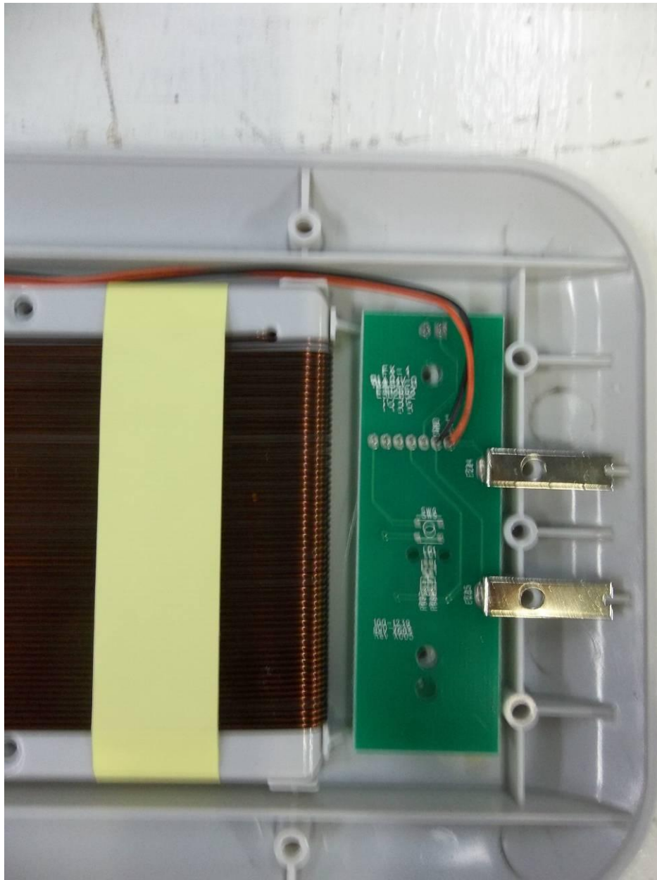
Figure 5. Close up of EUT with # 3 Cover Removed
