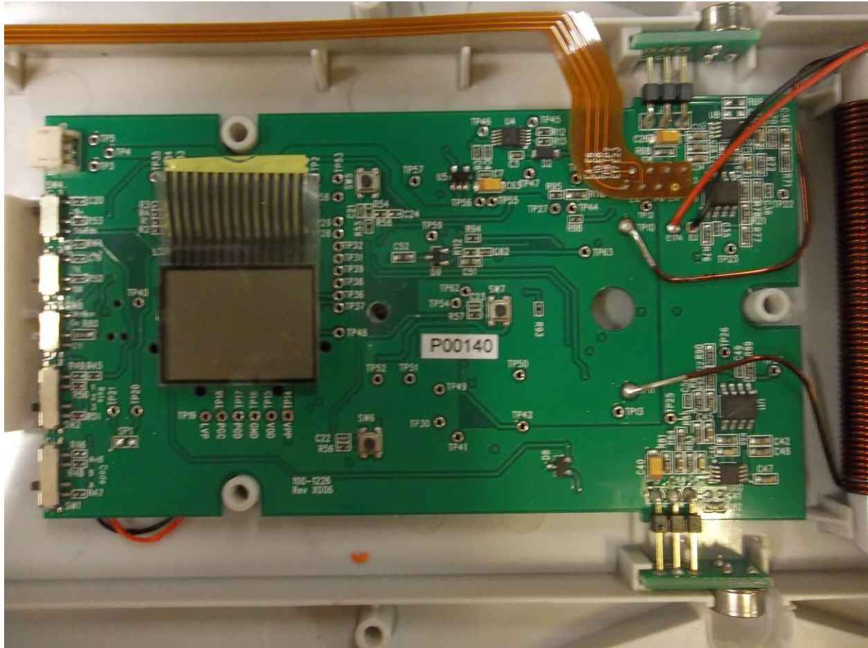
Figure 8. Front of PCB with Radio
