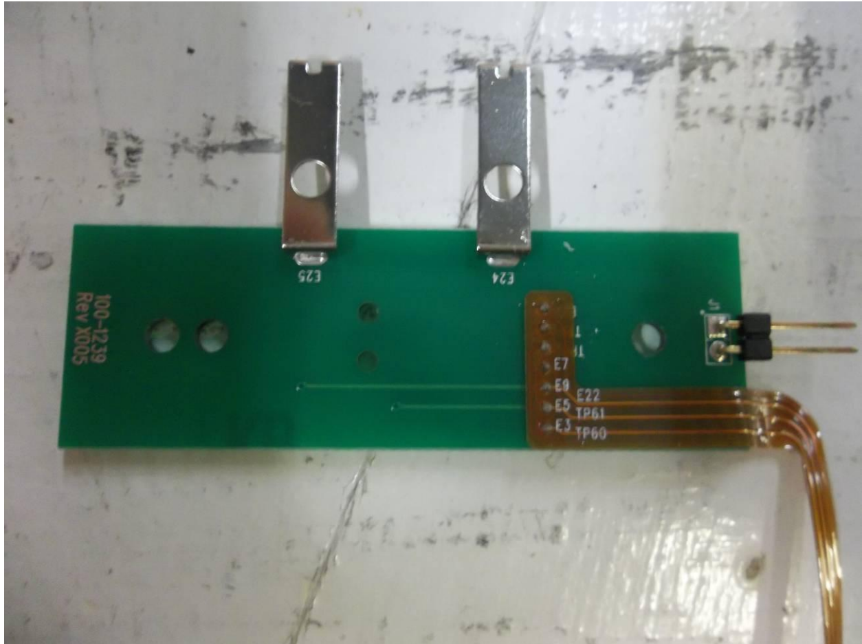
Figure 7. Back of PCB #1
