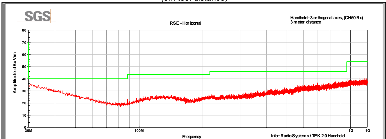
Channel 50 (Rx Mode) 30-1000MHz Horizontal (3m test distance)
