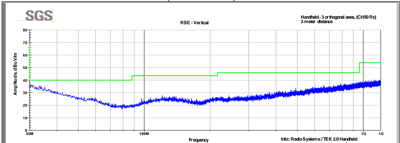
Channel 50 (Rx Mode) 30-1000MHz Vertical (3m test distance)
