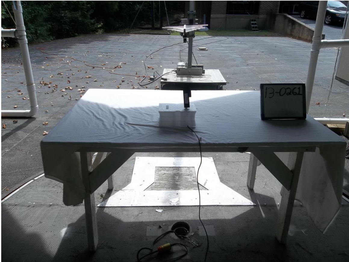
Figure 2. Rear View Radiated Emissions Test Setup
