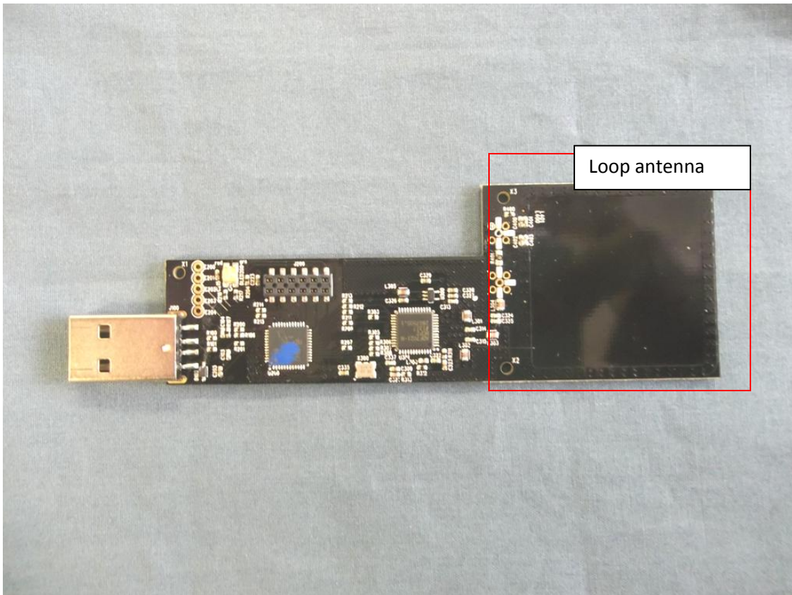
Figure 2. Component Side of EUT PCB
