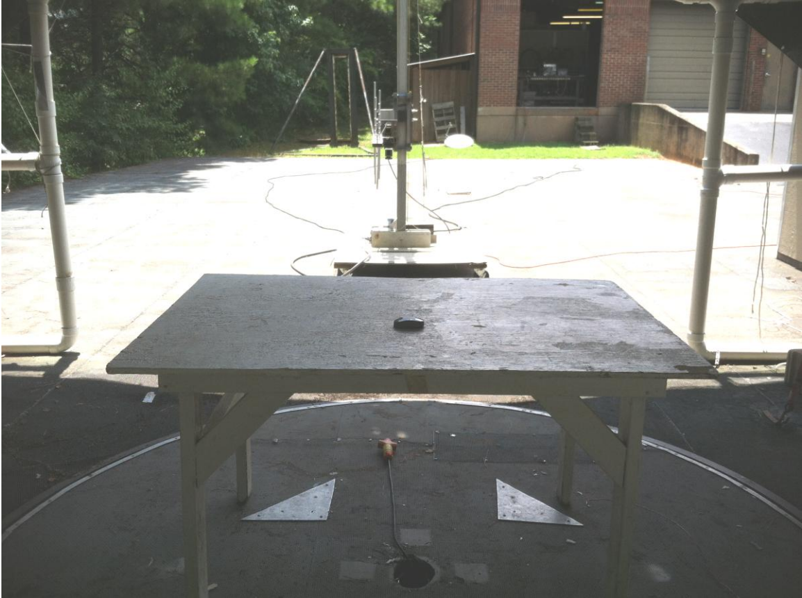
Figure 4. Radiated Emissions Test Setup (between 200 - 1000 MHz)
